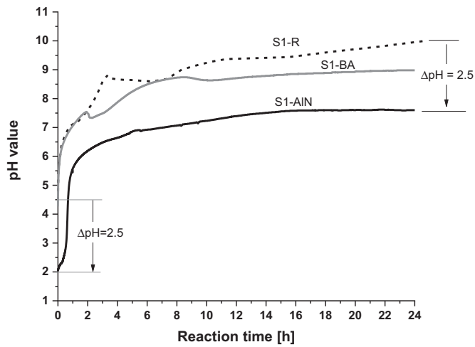
Fig. 2. Evolution of pH in the cement suspensions without (S1-R)/with aluminum nitrate (S1-AlN) or boric acid (S1-BA) at 20 mmol/L. Data are taken from [7] for S1-R.
