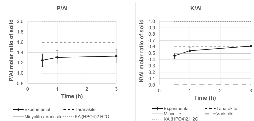
Fig. 8. Comparison of the P/Al and K/Al molar ratios of the solid formed during the first 3 h of hydration with those of well-known aluminophosphate minerals (Variscite AlPO_4 \cdot 2H_2O , Taranakite K_3Al_5H_6(PO_4)_8 \cdot 18H_2O , OH-Minyulite KAl_2(PO_4)_2(OH) \cdot 4H_2O , and KAl(HPO_4)_2 \cdot H_2O ).
