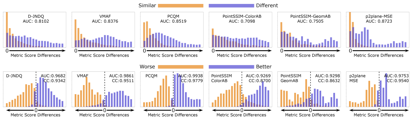
Fig. 8. The plots in the top row depict the metric score differences for pairs categorized as “Different” and “Similar” for the Intra-SRC evaluation. Each metric’s score differences are individually normalized within minimum and maximum ranges. The height of the bars represents the number of occurrences, and each bar ranges between 0 and 1500. The metric names are indicated at the top of each plot, and the AUC values are reported below each metric name. Similarly, the plots in the bottom row show the metric score differences for pairs categorized as “Better” and “Worse” for the Intra-SRC evaluation. Again, the metric score differences are individually normalized within minimum and maximum ranges. The height of the bars denotes the number of occurrences, and each bar ranges between 0 and 800. The metric names are indicated at the top left corner of each plot and the AUC and CC are reported in the top right corner of each plot.
