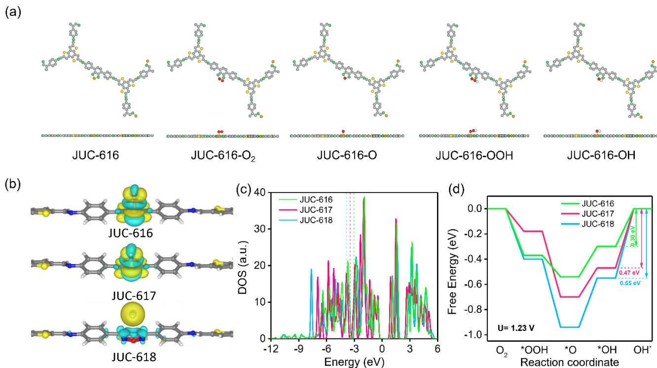
Fig. 3. (a) Models for the adsorption of different ORR reaction intermediates by JUC-616. The grey, green, yellow, red, orange and white spheres represent C, N, S, O, Se and H atoms, respectively. (b) The charge distribution of JUC-616. The curly, silvery white, green and yellow spheres represent C, N, Se and S atoms, respectively. Free energy diagrams of Se, S, O atoms in JUC-616, JUC-617 and JUC-618 at the applied potentials of 0 V (c) and 1.23 V (d), respectively.
