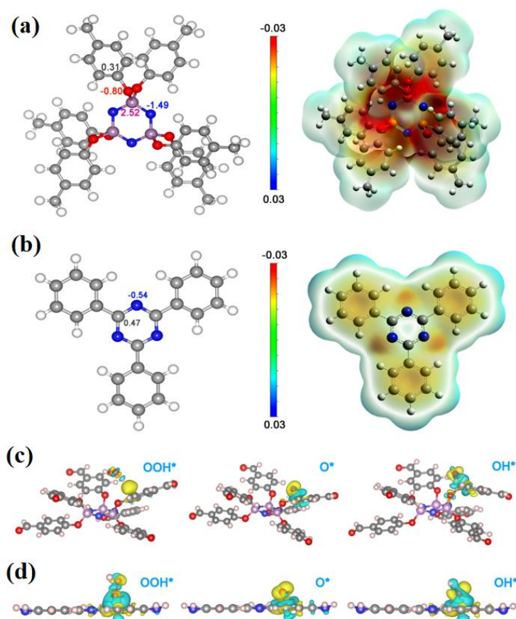
Fig. 4 a and b The NPA charges and the corresponding surface electrostatic potential maps of CTP-6-CHO and TAPT calculated by DFT. c and d Side view of the 3D charge densities for the three ORR reaction steps of C site for CTP-6-CHO and TAPT.
