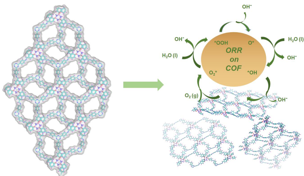
Scheme 2. Proposed ORR processes on JUC-610-CON.
