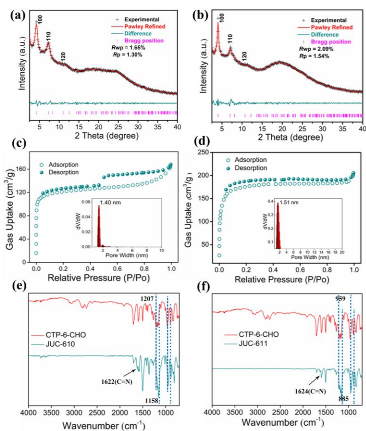
Fig. 1 a and b Powder XRD patterns of JUC-610 and JUC-611. c and d N_2 adsorption-desorption isotherms at 77 K and pore-size distribution (inset) based on the NLDFT model to the adsorption data for JUC-610 and JUC-611. e and f The FT-IR spectra of JUC-610 and JUC-611.
