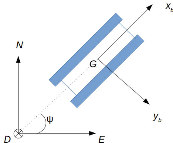
FIGURE 2 – Coordinates systems
