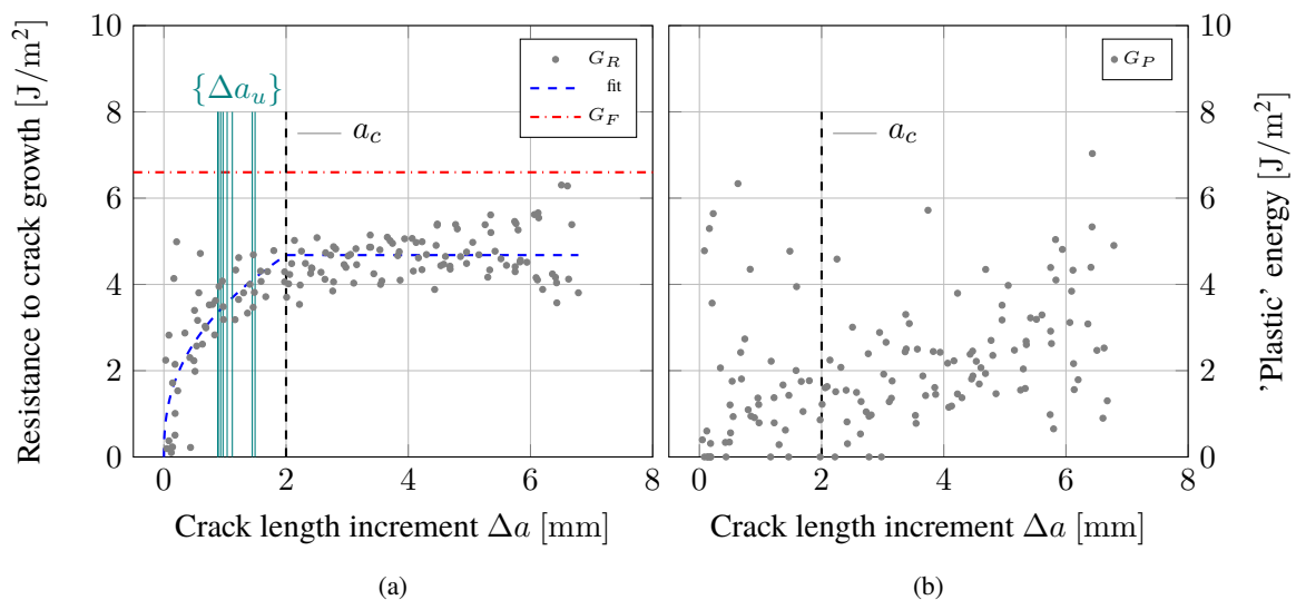
FIGURE 6 – Final R-curve for the ACP (a) and its corresponding 'plastic' energy curve (b).
