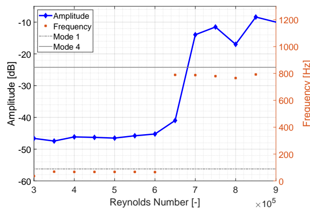
FIGURE 4 – Amplitude and frequency of the dominant peak in the response spectrum as a function of the Reynolds number, for α = 8°.
