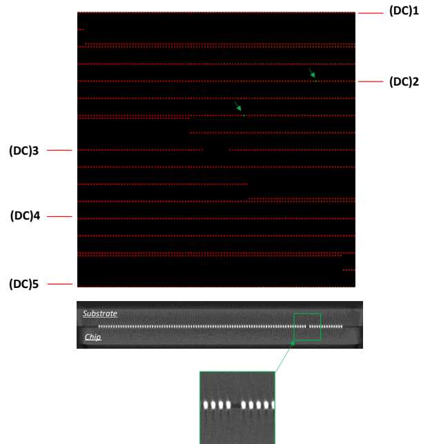
Fig. 5. Reconstruction after tomography X analyses of functional DCs (green) and dysfunctional DCs (red), showing two missing pillars correlating with only 3 functional DCs.
