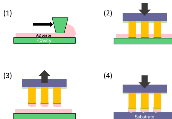
Fig. 3. Steps of the dip-transfer process in order to obtain silver sintered flip-chip assembly.
