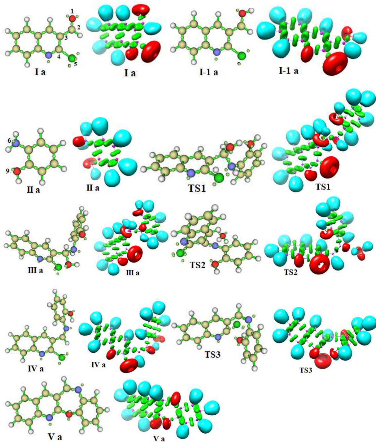
Figure 5. ELF localisation domains, represented with an isosurface value of ELF = 0.83 and basin attractor positions, monosynaptic basins are colored in red, di-synaptic basins are colored in green and protonated di-synaptic basins C-H and X-H are colored in blue.
