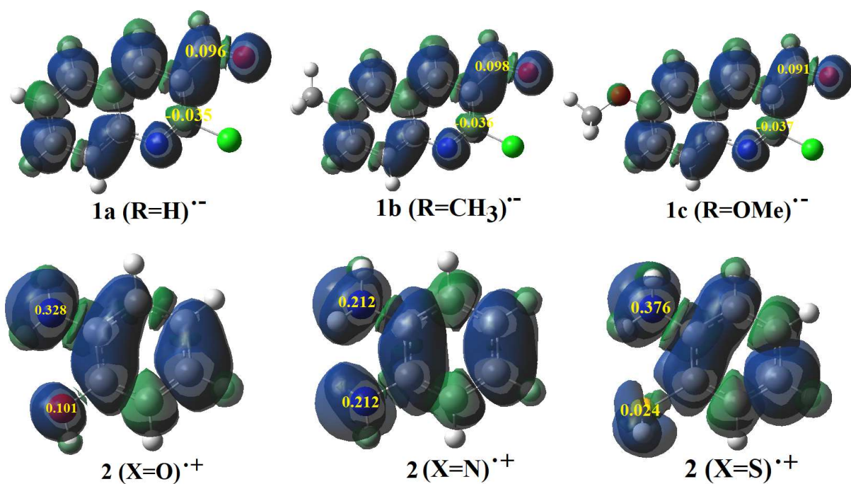
Figure 1. 3D representations of the ASD of the radical cation 2(X=O, N, S)^{\bullet+} and the radical anion 1a-c^{\bullet-} , as well as the nucleophilic and electrophilic Parr functions of 2(X=O, N \text{ and } S) and 1a-c .
