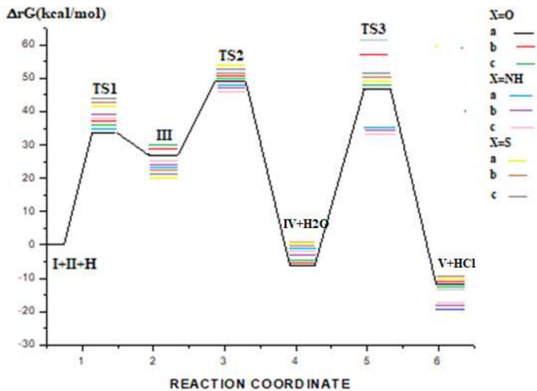
Figure 4. Evolution of the free enthalpy during the reaction mechanism
