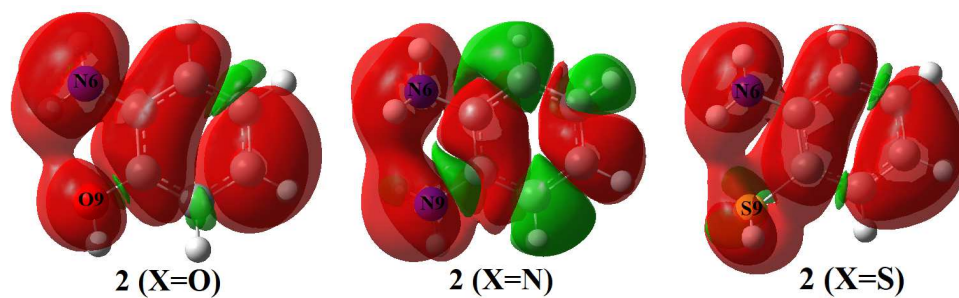
Figure. 2. The isodensity map of the dual descriptor \Delta f(r) calculated for reactants 1a-c and 2(X=O, N, S), \Delta f(r) > 0 colored in green and \Delta f(r) < 0 colored in red.
