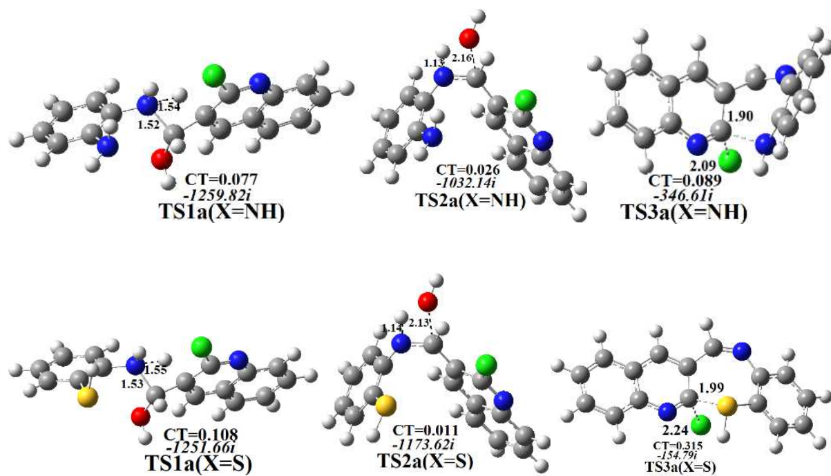
Figure 3. B3LYP/6-31G(d) geometries of the TS a(X=O, NH,S) structures, (length in Angstroms Å, and charge transfer values in e).
