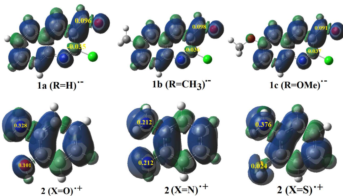
Figure. 1. 3D representations of the ASD of the radical cation 2(X=O, N, S) \cdot^+ and the radical anion 1a-c \cdot^- , as well as the nucleophilic and electrophilic Parr functions of 2(X=O, N \text{ and } S) and 1a-c .
