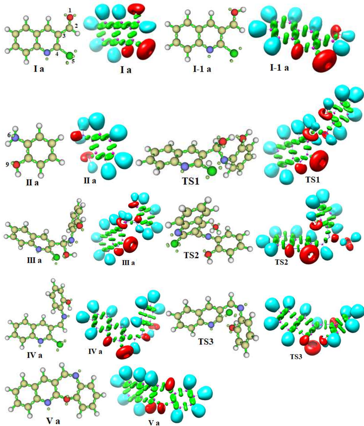
Figure 5. ELF localisation domains, represented with an isosurface value of \text{ELF} = 0.83 and basin attractor positions, monosynaptic basins are colored in red, di-synaptic basins are colored in green and protonated di-synaptic basins C-H and X-H are colored in blue.
