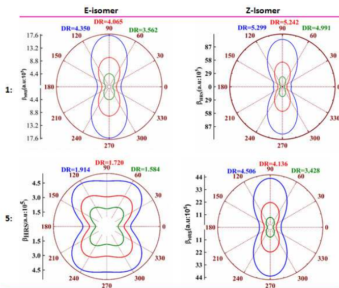
Figure 11. Relationship between I_{\Psi\Psi}^{2\omega} and polarization angle \Psi of Z and E isomers (green static, red \lambda = 1340 nm, blue \lambda = 1064 nm)
