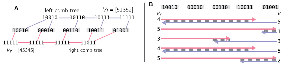
Figure 2. (A) Two Bloom comb trees and their Aggregated Bloom filters. The leaves Bloom filters are in the middle, colored in grey. They are the Bloom filters representing the input datasets. The left-comb tree (top) and right-comb tree (bottom) are built by aggregating the Bloom filter's k -mers. The Aggregated Bloom filter V_l represents the leftmost path of the top comb. Respectively, V_r represents the rightmost path of the bottom comb. We colored in green the second bit of leaves in order to show its encoding in the Aggregated Bloom filters. In the left comb, this bit is set to 1 only in the root for the longest branch; therefore, the value is 1 (green) in V_l . Conversely, the longest branch of the right tree has a run of five 1's on the second position, hence, a 5 in V_r . (B) Using V_l and V_r from (A), we show how Aggregated Bloom filters define restrained search spaces in the leaves. Again, the leaves' Bloom filters are grey, and the values of the vectors are printed vertically. Arrows represent the intervals given by each V_l and V_r , and the final search space at each position is the dotted grey area.
