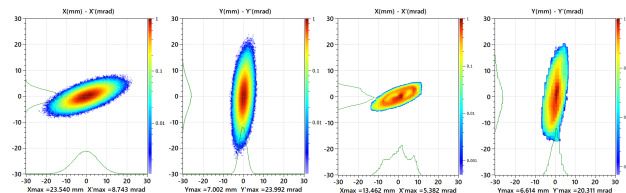
Figure 2: Transversal phase space in the MEFT for 0.7 mA {}^{18}O^{6+} beam: reference simulation (left) and measurement (right).
