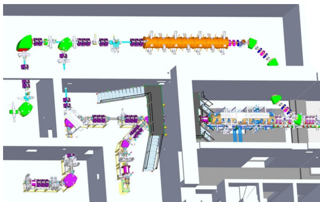
Figure 6: SPIRAL2 NEWGAIN injector.
