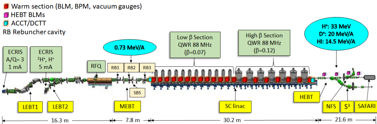
Figure 1: SPIRAL2 SC linac layout.
