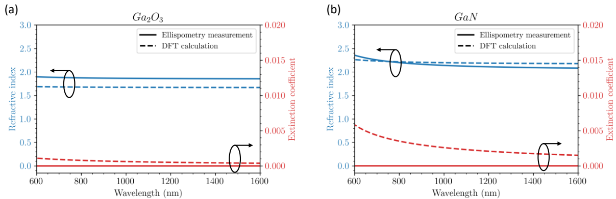
Figure 4: Optical properties of \text{Ga}_2\text{O}_3 and GaN ultrathin films, extracted from spectroscopic ellipsometry and DFT in the range 600–1600 nm. (a) Shows the refractive index n and extinction coefficient k of \text{Ga}_2\text{O}_3 as a function of wavelength, (b) shows the refractive index n and extinction coefficient k of GaN as a function of wavelength.
