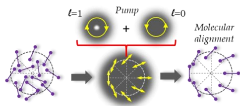
Fig. 3 Illustration of the mechanism for storing \ell = 1 OAM state. The global pump field exhibits an azimuthal distribution of polarization inducing a molecular alignment along the same pattern (equivalent to a q-plate with q = 1/2 ).
