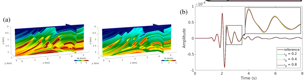
Figure 4 (a) 3D Marmousi-II velocity models without the water layer which is used to calculate the reference solution for benchmarking against the homogenized solutions, (b) seismogram comparison of vertical displacement generated from (a) and the effective models with \epsilon_0 = 0.2, 0.4 and 0.8 in Figure 5.
