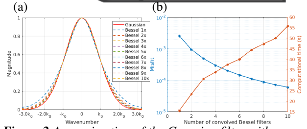
Figure 2 Approximation of the Gaussian filter with a cascade of Bessel filters (a) and the superposition (b) of the approximation accuracy (blue) and computational cost (orange) with respect to the number of Bessel filters (each one corresponds to a stretching factor \alpha calculated by PSO).
