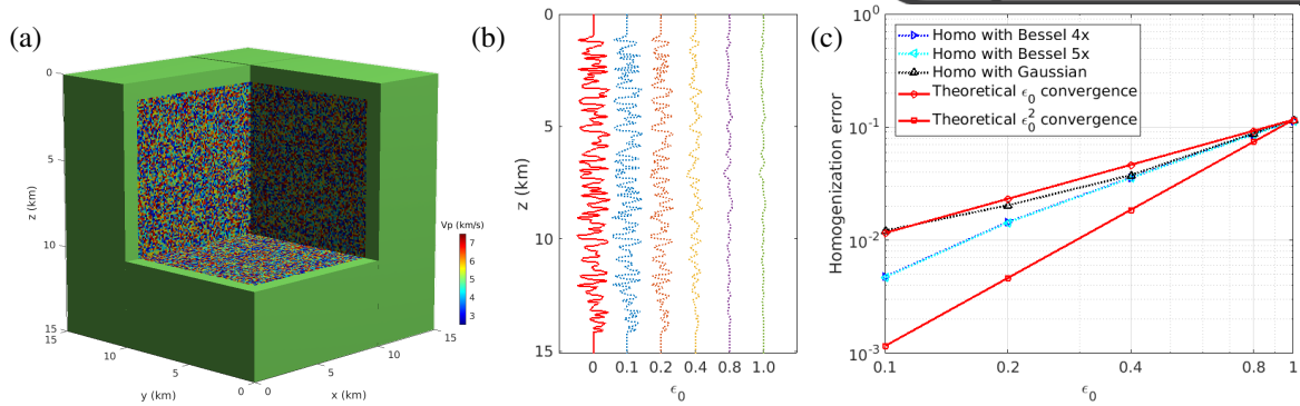
Figure 3 Homogenization test in a random medium. (a) The random P-wave velocity model V_p , (b) 1D V_p profiles of the random model (red solid line) and the effective models using 4 Bessel filters with different \epsilon_0 (dash lines), (c) the convergence history of the wavefields generated from the effective models with respect to \epsilon_0 and the type of low-pass filters (Gaussian filter and its approximation through Bessel filters).
