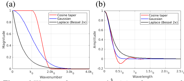
Figure 1 Wavenumber spectra \hat{w}^{\lambda_0} (a) and corresponding wavelets w^{\lambda_0} (b) for three low-pass filters: Cosine-tapered filter, Gaussian filter and Laplace filter implemented by cascading two Bessel filters, with 2.5\lambda_0 spatial support.
