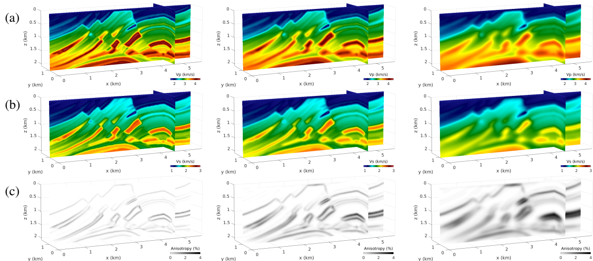
Figure 5 3D Marmousi-II effective models with \epsilon_0 = 0.2, 0.4 and 0.8 from left to right. (a) P-wave velocity model ( V_p ), (b) S-wave velocity model ( V_s ) and (c) the total anisotropy in percentage, which are calculated by projecting the resulting C_{ijkl} from homogenization to the closest isotropic model (Browaeys and Chevrot, 2004).
