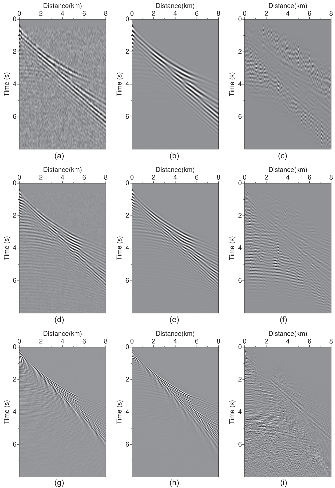
Figure 21. The observed data: 2–4 Hz (a), 2–6 Hz (d) and 2–15 Hz (g). The calculated data (b, e, h) with the reconstructed models using data on the left-hand side. The pictures (c, f, i) on the 3rd column display the corresponding adjoint sources of LAWI for the first iteration, which indicates that LAWI can gradually take reflections into account with multi-scale strategy.
