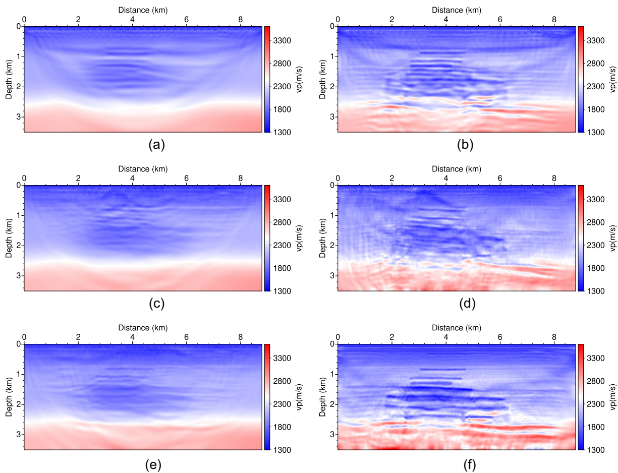
Figure 20. Inversion results starting with the third velocity model and a smooth density model. Pictures on the left-hand side show the recovered velocity models computed with weighted data after 20 iterations: (a) FWI, (c) AWI and (e) LAWI. Pictures on the right-hand side show the recovered velocity models subsequently computed with full data after 50 iterations: (b) FWI, (d) AWI and (f) LAWI.
