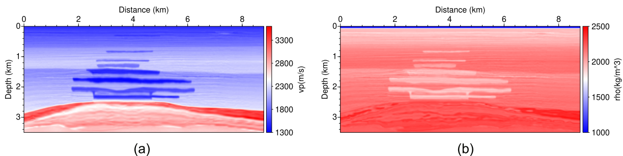
Figure 8. 2-D Valhall models: (a) P-wave velocity model, (b) density model.
