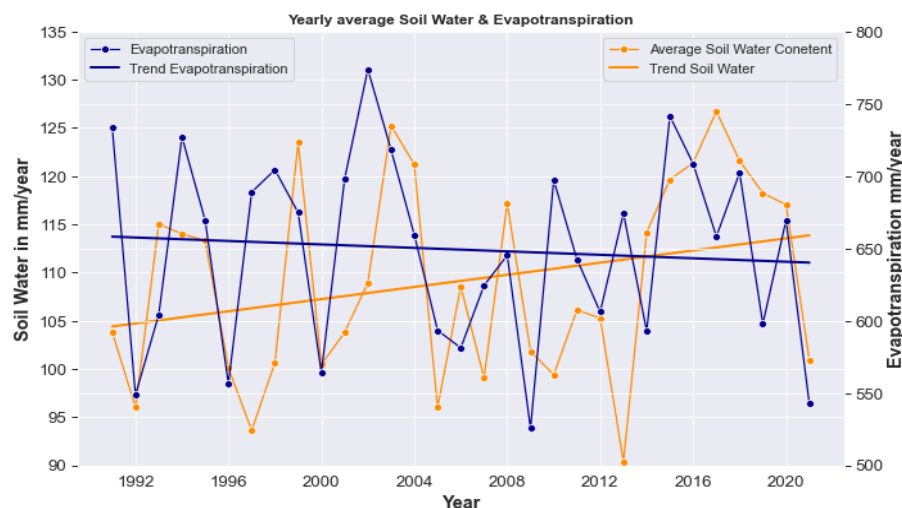
Figure 14. Yearly average soil water content and evapotranspiration in mm with their respective linear regression curves.
