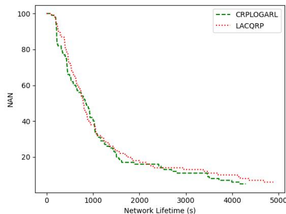
Fig. 3. Number of alive sensors with network lifetime.
