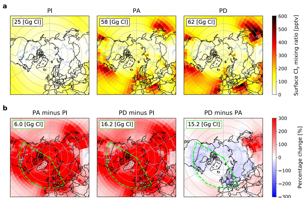
Figure 3. 30°–90°N regional distributions of annual-mean surface mixing ratios of Cl y in the three-time periods in GEOS-Chem (a), and the percentage difference of Cl y surface mixing ratio between the three-time periods (b). Gray grid lines show 10° latitude and 60° longitude distance. Black crosses mark the ice-core sites. Dashed green lines show the back trajectory region (TRJ, 120°W–30°E, 42°–90°N) for the six Greenland ice cores based on the 5-day back trajectory analysis. The annual-mean tropospheric Cl y burdens for 30°–90°N regions are shown on the top-left corners of subplots in (a), and the burdens for the TRJ region are shown similarly in (b).
