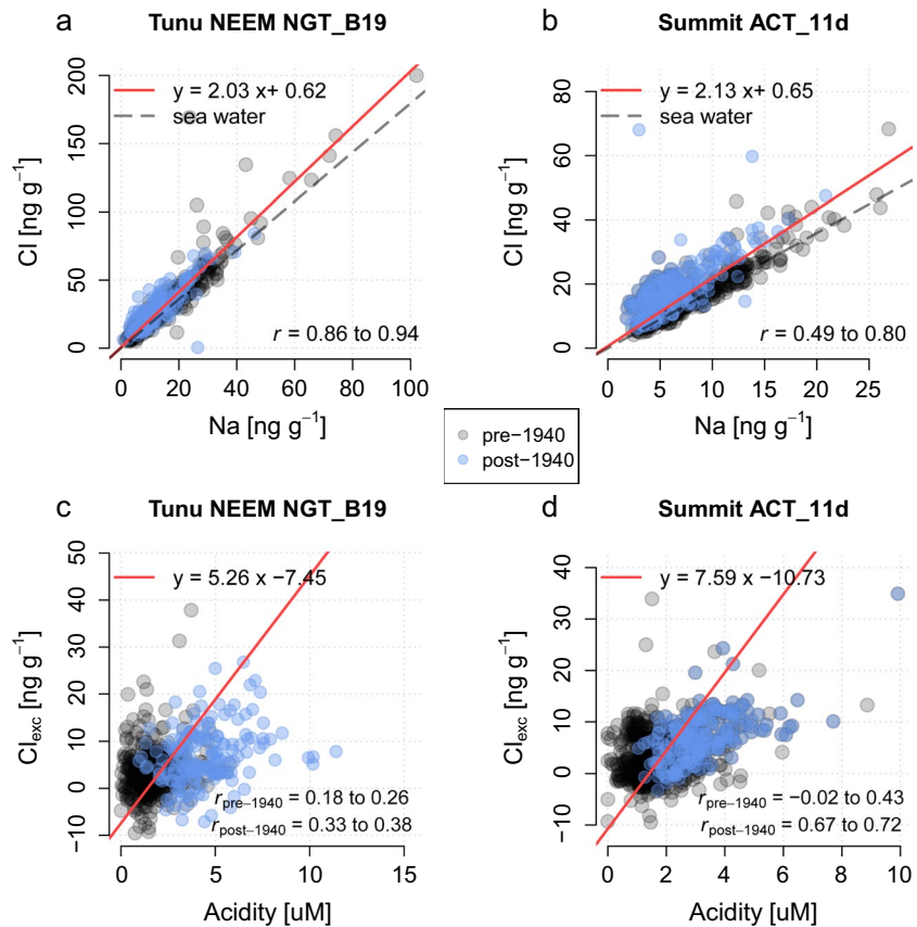
Figure 2. Relationships between annual ice-core (a and b) Na and Cl concentrations, and (c and d) snow acidity and Cl_{exc} from the six Greenland ice-core records. (a and c) Higher latitude cores including Tunu, NEEM, NGT_B19, (b and d) the lower latitude cores including Summit07, Summit10, and ACT_11d. Black circles are the pre-1940 record and blue circles represent post-1940 records. Red lines and the equation show the PB regression for the full record. Dashed black lines show the relationship between Na and Cl in sea water. r , r_{pre-1940} , and r_{post-1940} represent, respectively, the Pearson's correlation coefficients for the full records, pre-1940 and post-1940 records, and the range of r values is from individual ice cores in the group. Outliers outside the 1.5 \times IQR (interquartile range) are removed. All r values are significant with p values lower than 0.05.
