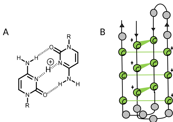
Figure 2. (A) (CH^+ \cdots C) base pairing, (B) schematic representation of i-DNA .
