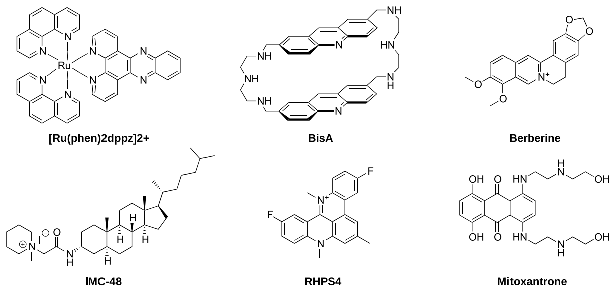
Figure 12. Structure of compounds used for the studies of i-motif interactions. [\text{Ru}(\text{Phen})_2\text{dppz}]^{2+} [66], BisA [67], Berberine [68], IMC-48 [19], RHPS4 [69] and mitoxantrone [70].
