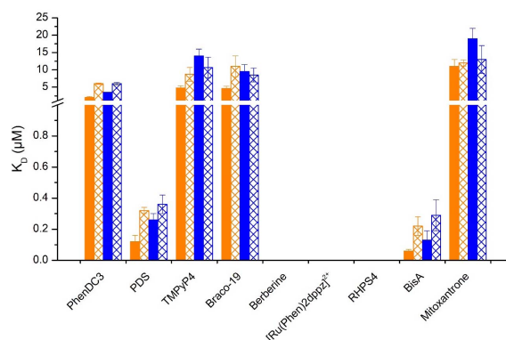
Figure 13. K_D values obtained with different ligands in interaction with I-motif 6 (blue), h-Telo sequence (orange) at pH 5.5 and 6.5 fill and sparse pattern. No histogram for duplex berberine, [\text{Ru}(\text{Phen})_2\text{dppz}]^{2+} and RHPS4 means that the K_D value could not be determined due to too weak interaction. The reported values are the means of representative independent experiments, and the errors provided are standard deviations from the mean. Each experiment was repeated at least three times.
