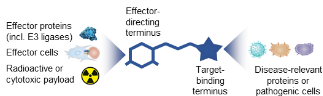
Figure 3. Chemical inducers of proximity are bifunctional molecules combining effector- and target-binding moieties, and are able to target a therapeutic effector to the immediate vicinity of a disease-related protein or pathogenic cell.
