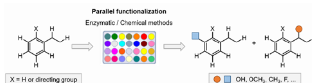
Figure 5. Directed as well as non-directed late-stage diversification methods can considerably accelerate access to new drug molecules. Figure reproduced under licence CC BY 4.0 from CHIMIA, 2022, 76, 258.
