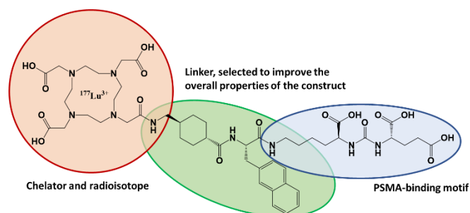
Figure 4. Structure of Pluvicto ® , illustrating the modulatory construction of RLTs.
