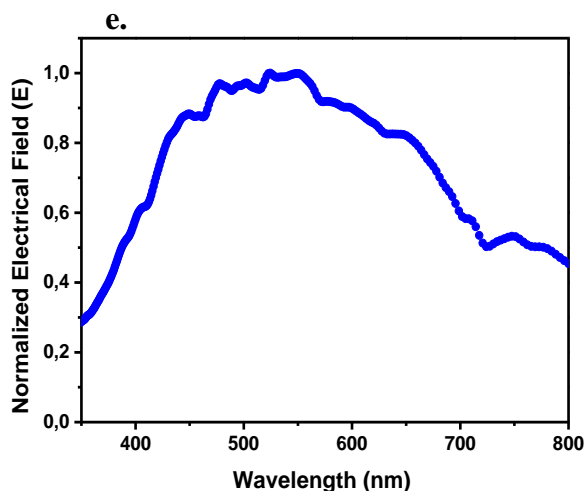
Figure 5: a. ZAZ Architecture simulated with Lumerical FDTD Solution; b. Related Reflection, Transmission and Absorption; ZAZ electrode electrical field simulated at 454 nm c. top view; d. cross section view; e. Normalized Electrical Field of Simulated ZAZ electrode.
