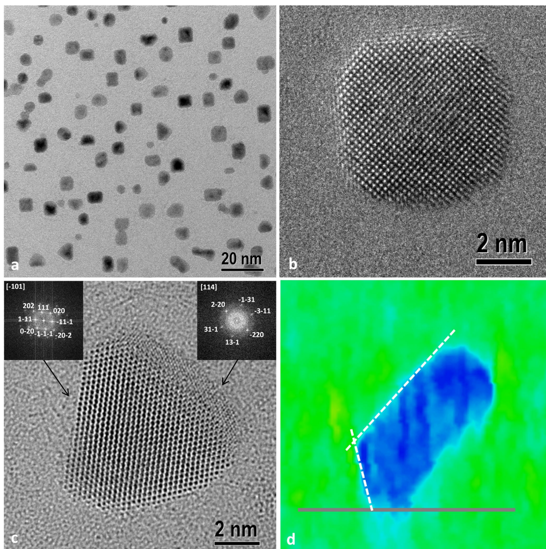
Figure 6 : (a) Bright field image of as-grown CoPt NPs obtained on a carbon replica. (b) HRTEM image of a CoPt NP oriented along the [002] showing the truncated octahedron morphology. (c) Triangular shaped NP exhibiting the [-\bar{1}01] and [114] zone axes orientations. (d) 3D shape of the triangular shaped NP obtained by electron tomography showing the angel wing like morphology. CoPt nanoparticle is in blue, vacuum is in green and the substrate plane is outlined by the horizontal grey line.
