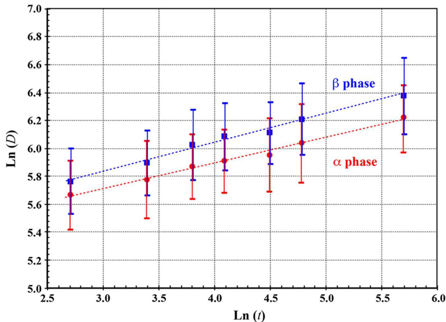
FIGURE 6 | Linear relationship between \ln(D) and \ln(t) for \alpha and \beta grain growth of Ti35-5-5 at 650°C.
