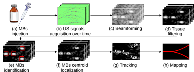
Fig. 1: ULM framework example.
