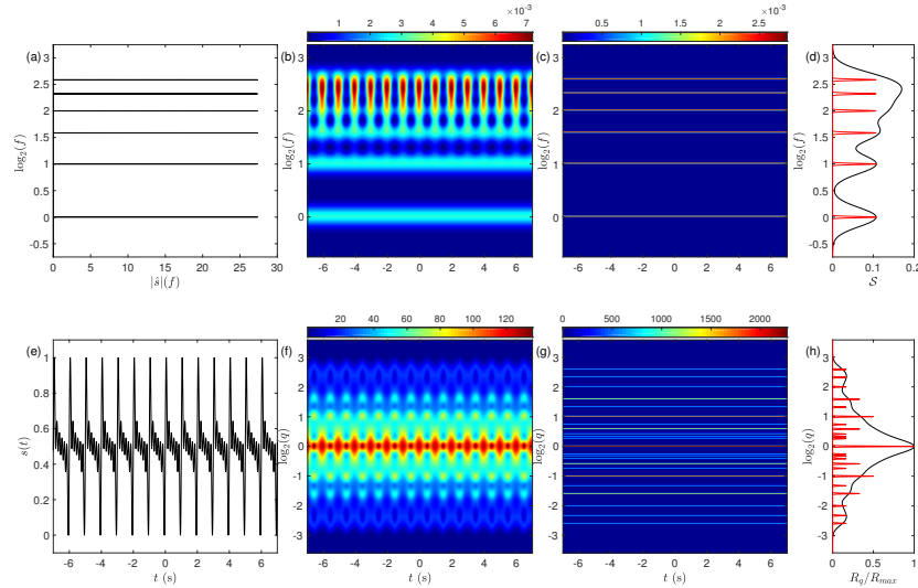
Fig. 5 Analysis of a model signal defined as the sum of 6 sine functions s(t) = \sum_1^6 \sin(2\pi f_i t) , with f_i = i f_1 constant. (a) Fourier spectra of s : |\hat{s}(f)| on which the two axes have been inverted. (b) S^{(8)}(\log f, t) , computed for Q = 8 . (c) S^{(128)}(\log f, t) , computed for Q = 128 . (d) S^{(Q)}(\log f, t = 0) . (e) Temporal signal s(t) in the time window [-6.5s, 6.5s] . (f) R[S^{(8)}, S^{(8)}](\log q, t) . (g) R[S^{(128)}, S^{(128)}](\log q, t) . (h) R[S^{(Q)}, S^{(Q)}](\log q, t = 0) . In (d) and (h) the plots for Q = 8 (resp. 128) are coloured in black (resp. red). R[S^{(Q)}, S^{(Q)}](\log q, t) is defined in Eq. (27).
