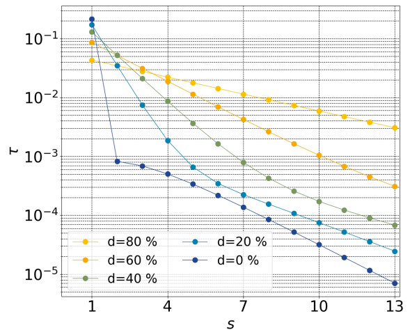
Figure 6. Evaluation of the virial convergence parameter defined in Eq. (19) \tau(s) = \left( \frac{T_F}{W_F} - \frac{T_F^c}{W_F^c} \right)^{(s)} as a function of the number of steps s of the self-consistent scheme for U/t = 4 . Results are provided for different number of dampings. Lines are guidelines for better visualization
