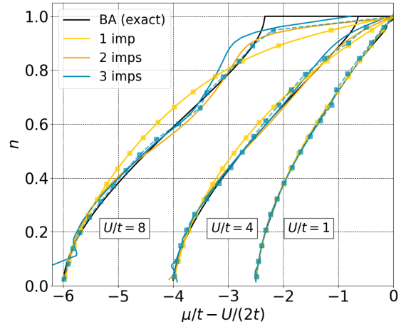
Figure 8. Lattice filling n with respect to the chemical potential \mu(n) = \partial E_{gs}/\partial n calculated for U/t = 1, 4, 8 . Results are provided for different numbers of impurities (full lines). Comparison is made with the exact Bethe Ansatz (black solid line). Squares and dashed lines correspond to interacting-bath DMET.
