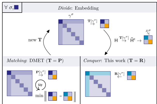
Figure 2. Representation of the Divide-and-Conquer protocol proposed in this work compared to the standard DMET self-consistent scheme.
