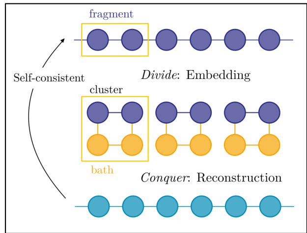
Figure 1. Schematic representation of the divide and conquer strategy.
