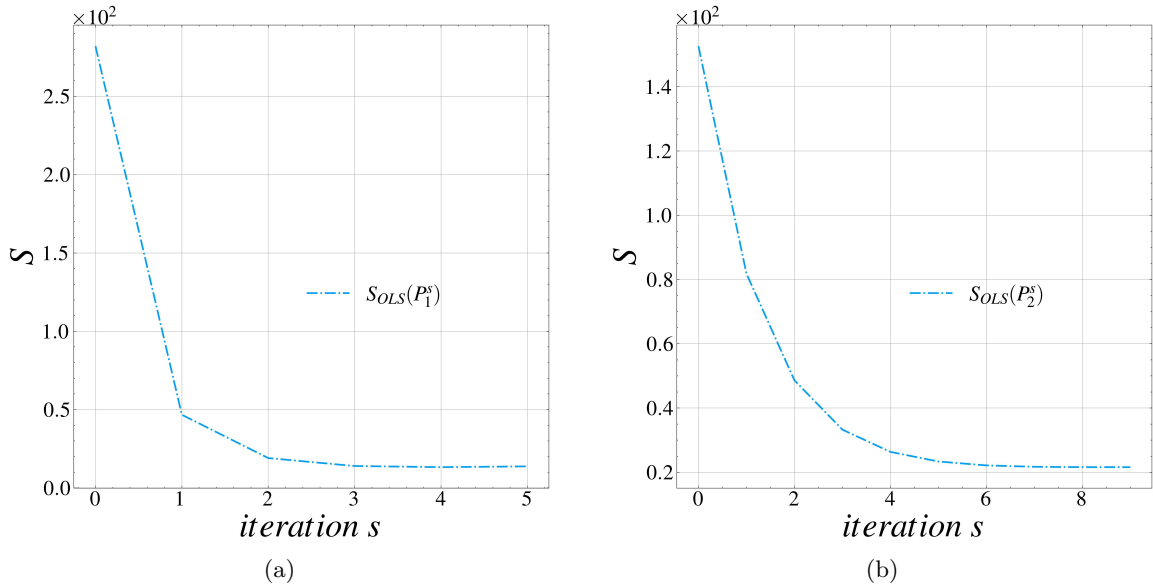
Figure 8. The variation of the objective function with respect to iteration for the first (a) and the second (b) materials.
