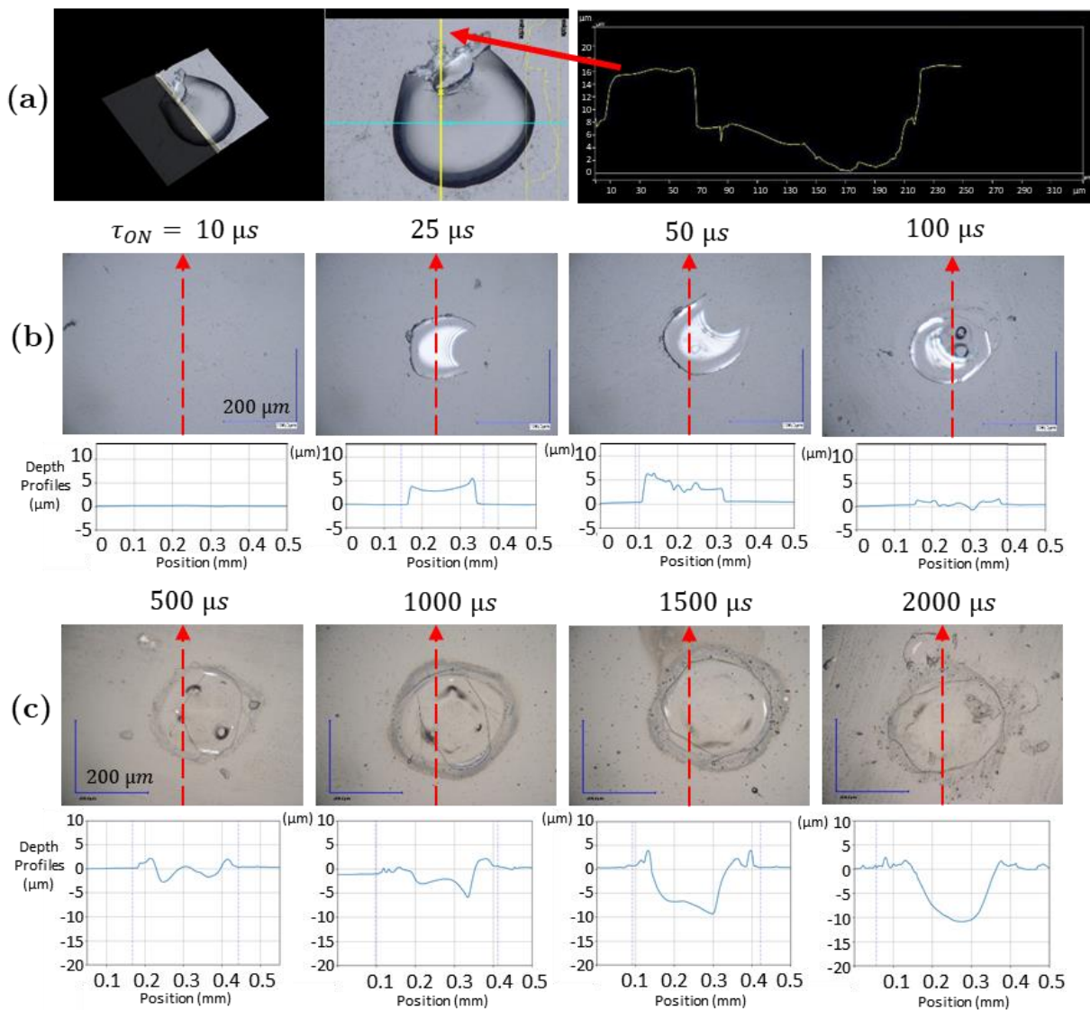
Fig. 5 Static irradiation damaged zones on SDL glass for increasing \tau_{ON} . Each picture scale and profile X-axis is displayed with the same scale factor (200 \mu m ). Each profile Y-axis is displayed with the same scale factor. Red arrows correspond to the profile measurement path. (a) The glass fragment has been removed by air blowing. This allowed 3D surface profile measurements with the KEYENCE. The profile on the right corresponds to the yellow arrow of the figure in the middle. (b) Microscope photograph and corresponding stylus profilometry. (c) Microscope photograph of damaged sites and corresponding stylus profilometry.
