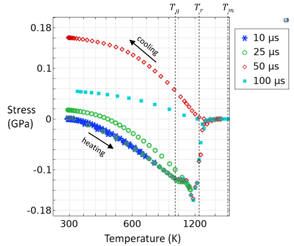
Fig. 9 Radial component of the transient stress \sigma_{rr} versus temperature at the surface center point. ( r=0, z=0 ) Vertical lines correspond respectively from left to right to the glass transition temperature, stress relaxation point (1250 K) and melting temperature. All traces correspond to different values of \tau_{ON} . Positive stress is tensile and negative is compressive.
