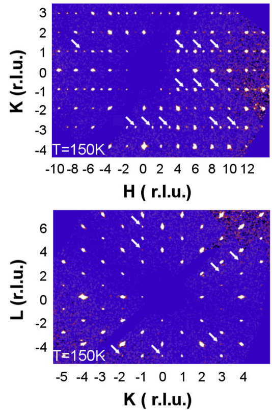
FIG. 2. Reconstructions of the lattice node planes ( H, K, 0 ) (up) and ( 0, K, L ) (down) of \text{BaFe}_2\text{Se}_3 (sample S1) at 150 K, taking into account absorption correction. Arrows in the down panel indicate the forbidden reflections associated with the \mathbf{n} glide planes.
