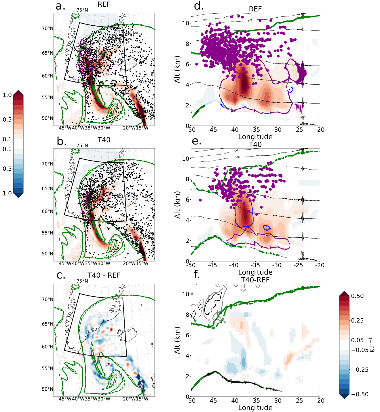
Figure 5. (Left panels) Vertically averaged heating rate between 2 km and 9 km (shadings) and (right panels) meridionally averaged heating rate (shadings) in the large black area shown in upper panels at 18 UTC 2 Oct for (a),(d) REF, (b),(e) T40 and (c),(f) the difference T40-REF. Black dots in (a),(b) correspond to WCB trajectories positions at 18 UTC 2 Oct, while the purple dots correspond to the trajectories ending in the red PV anomaly shown in Fig. 4a. In the upper panels one trajectory in five are represented for visibility sake. Green lines represent the position of the dynamic tropopause (full line in REF and dashed line in T40). The grey and black lines in (f) represent the 1 PVU and 0.5 PVU difference between T40 and REF (solid lines for positive values and dashed for negative ones). The purple and blue contours in (d),(e) represent the CDEPI and DEPS contributions (see Table 1 for their definition) respectively when it is greater than 0.3 \text{ K.h}^{-1} (solid for positive values and dashed for negative ones).
