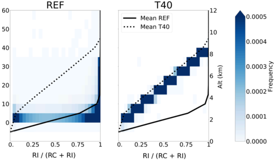
Figure 2. Bivariate PDFs as a function of temperature for partition of pristine ice over sum of cloud droplets and pristine ice over the whole domain using forecast time after 12, 18, 24, 36, 48 hours for the stalactite cyclone simulation initialized at 00 UTC on 1 Oct. Zero value for mixing ratio is not considered in bivariate PDFs calculation. REF is on the left, T40 is on the right, mean values of the ratio are plotted in solid lines for REF and dashed lines for T40.
