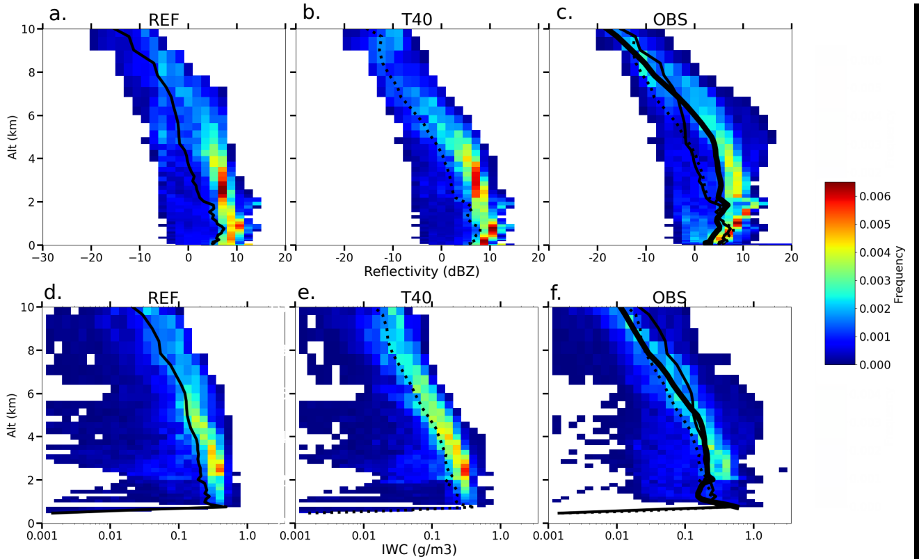
Figure 11. During F15 Thor ridge, Bivariate PDFs as a function of altitude of (a)-(c) radar reflectivity and (d)-(f) Ice Water Content for (a),(d) REF, (b),(e) T40 and (c),(f) the observations regridded onto the model grid, mean vertical profiles are indicated for REF (solid line), T40 (dashed line), and observations (thick solid line). The measurements and observations are normalized with the total number of points.
