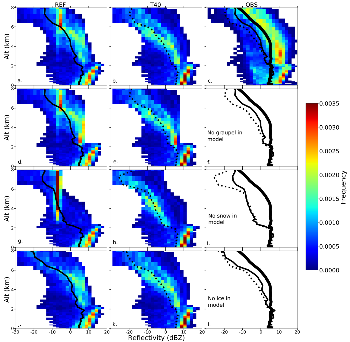
Figure 9. During F7 (stalactite cyclone), bivariate PDFs as a function of altitude of radar reflectivity (a)-(c) total hydrometeors, (d)-(f) without graupel in model, (g)-(i) without snow in model, (j)-(l) without ice in model, (a),(d),(g),(j) REF, T40 and (c),(f),(i),(l) the observations regridded onto the model grid, mean vertical profiles are indicated for REF (solid line), T40 (dashed line), and observations (thick solid line). The measurements and observations are normalized with the total number of points. The simulations are initialized at 00 UTC 1 Oct.
