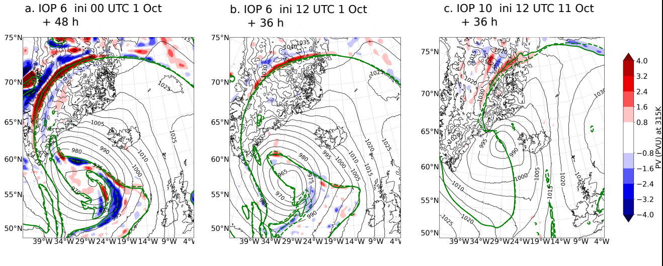
Figure 4. (a)-(c) PV differences between T40 and REF at the 315-K isentropic surface (shading; units: PVU) and SLP at (a-b) 00 UTC 3 Oct and (c) 00 UTC 13 Oct. The initial conditions are (a) 00 UTC 1 Oct, (b) 12 UTC 1 Oct and (c) 12 UTC 11 Oct.
