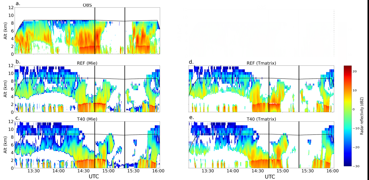
Figure 8. Along F7 (stalactite cyclone), reflectivity for (a) RASTA observations regridded onto the model grid, as calculated with the Mie scattering theory for (b) REF and (c) T40, as calculated with the T-matrix scattering theory for (d) REF and (e) T40. The vertical dark lines stand for the time where the flight changed direction. The simulations are initialized at 00 UTC 1 Oct.
