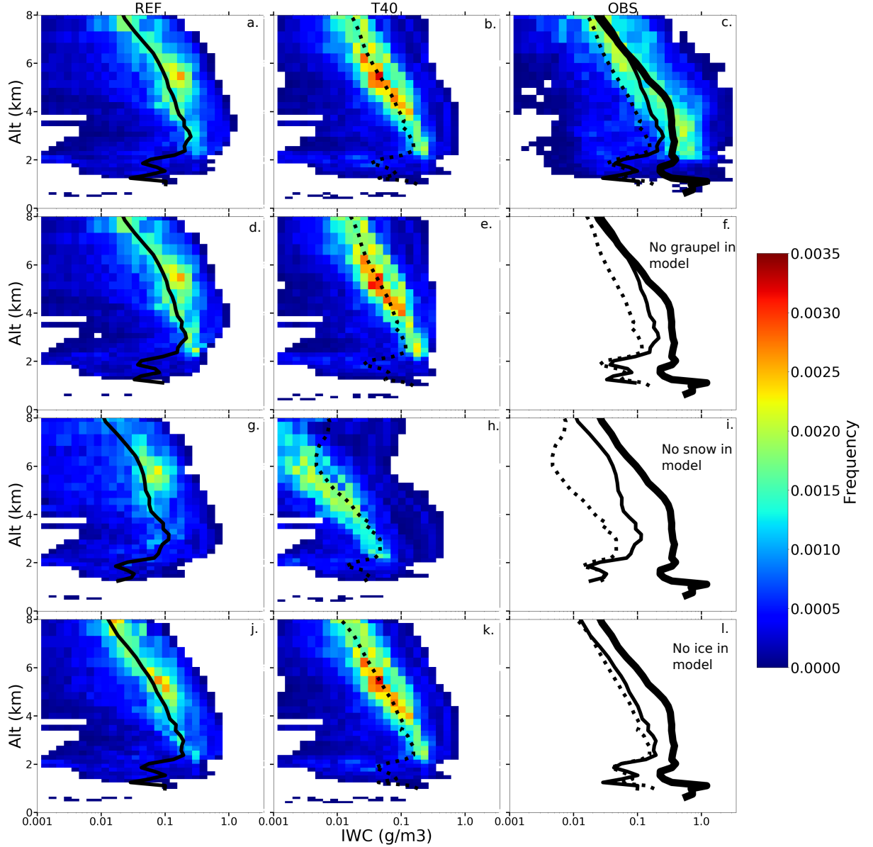
Figure 10. During F7 (stalactite cyclone), bivariate PDFs as a function of altitude of IWC (a)-(c) total hydrometeors, (d)-(f) without graupel in model, (g)-(i) without snow in model, (j)-(l) without ice in model, (a),(d),(g),(j) REF, (b),(e),(h),(k) T40 and (c),(f),(i),(l) the observations regrided onto the model grid, mean vertical profiles are indicated for REF (solid line), T40 (dashed line), and observations (thick solid line). The measurements and observations are normalized with the total number of points.
