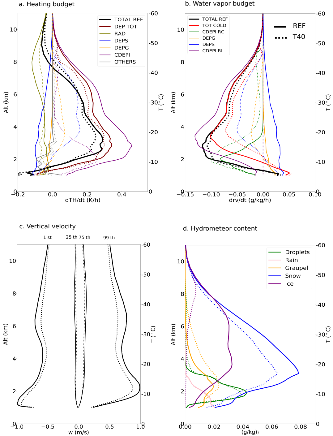
Figure 6. (a) Horizontal average of the heating rate over the box defined in Figs. 5a-c at 18 UTC 2 Oct for total absolute values greater than 0.0 \text{ K.h}^{-1} . In (b), (c) and (d) statistics are made over the same area and the same time as in (a). Only the main processes are plotted and explained in Table 1, OTHERS corresponds to the sum of all the other processes. (b) Horizontal average of the vapor mixing ratio tendencies. CDEPI RC/DEPG/DEPS/CDEPI RI correspond to deposition of vapor on droplets/graupel/snow/pristine ice respectively. TOT COLD combines all the cold processes. Total is the sum of all the tendencies. (c) 1st, 25th, 75th and 99th percentiles of the vertical velocity distribution. (d) Horizontal average of hydrometeor mixing ratios: RCT, RRT, RGT, RST and RIT correspond to droplets, rain, graupel, snow and ice mixing ratios. Full lines stand for REF and dotted ones for T40.
