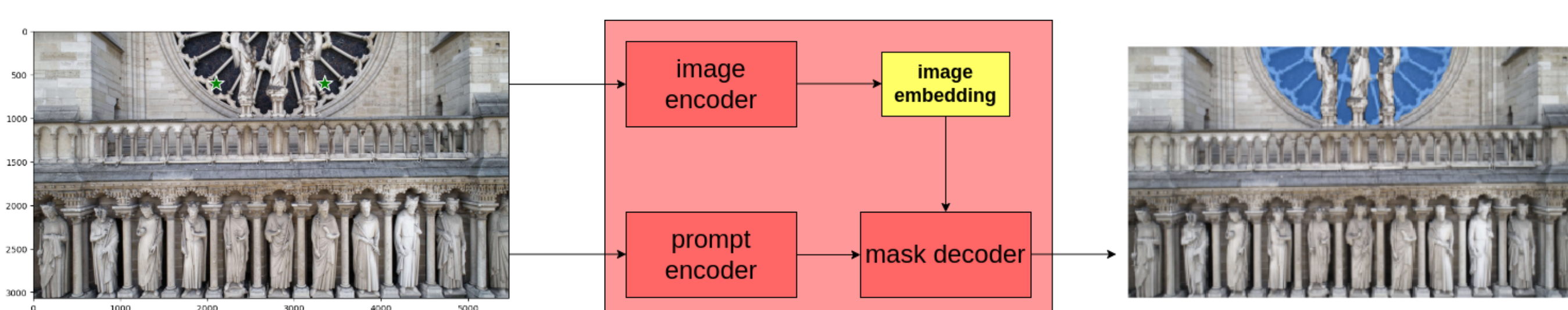
Figure: Overview of the Segment Anything Model.
