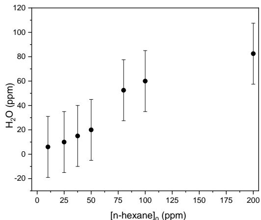
Fig. 6 Measurement of H 2 O mixing ratio at the exit of the DBD for mixing ratios of n-hexane in air up to 200 ppm (SED: 225 J/L, applied voltage: 23.4 kV, HV-pulse repetition frequency: 500 Hz, gas flow rate: 0.5 L/min).
