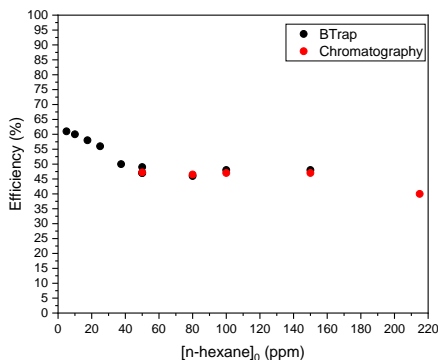
Fig. 4 Efficiency of the degradation of n-hexane as a function of the mixing ratio of n-hexane injected (SED = 265 J/L, applied voltage: 24.3 kV, HV-pulse repetition frequency: 500 Hz, gas flow rate = 0.5 L/min) .
