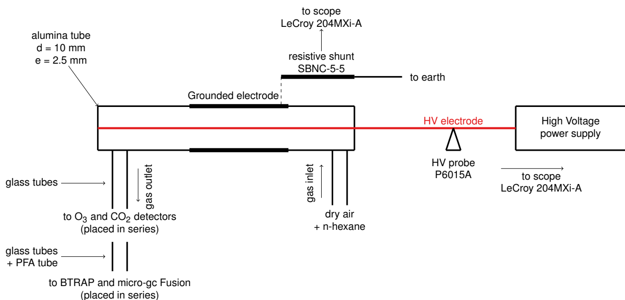
Fig. 1 Schematic drawing of the experimental set-up.
