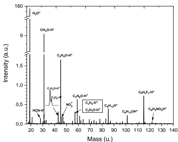
Fig. 8 Mass spectra obtained for the H_3O^+ precursor ion for an n-hexane mixing ratio of 100 ppm, with C_6H_4F_2^+ being used as an internal mass calibrant ( m/z 114.028).
