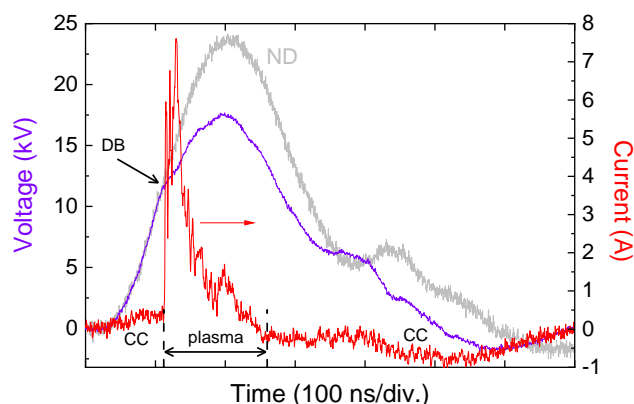
Fig. 2 Typical temporal evolutions of current and voltage. HV-pulse repetition frequency: 500 Hz, applied voltage: 23.6 kV (ND: no discharge, voltage plot in grey line), gas flow rate: 0.5 L/mn NTP, n-hexane mixing ratio: 100 ppm. DB: discharge breakdown, CC: capacitive current.
