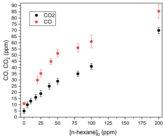
Fig. 5 Measurement of CO 2 mixing ratio (black) and CO mixing ratio (red) at the exit of the DBD for mixing ratios of n-hexane in air up to 200 ppm (SED: 225 J/L, applied voltage: 23.4 kV, HV-pulse repetition frequency: 500 Hz, gas flow rate: 0.5 L/min). Measurements are obtained using different detectors: CO by gas chromatography and CO 2 by IR detector.
