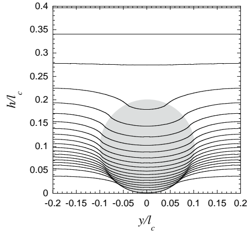
FIG. 2 – A unit cell for the periodic defect pattern (the area of a defect is shadowed) and periodic (both in time and space) solution of Eq. (6). 20 snapshots of the contact line with the equal time intervals 0.2\xi l_c/\sigma are shown for v = 0.1\sigma/\xi . The chosen parameters of the defect pattern are 2L = 0.4l_c , r = 0.1l_c , \theta_s = 70^\circ , and \theta_d = 110^\circ . The full picture of the contact line motion can be obtained by periodic continuation of this image in both vertical and horizontal directions.
