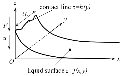
FIG. 1 – Reference system to describe the Wilhelmy balance experiment. The Wilhelmy plate is positioned in yOz plane. The positive directions for u and F are shown too.
