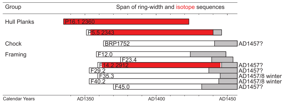
Figure 4. Bar diagram of the absolute dating of the original ring-width series (black outline with sapwood shaded grey) and isotope series (red) for the two hull plank samples, and framing timbers group NewportT7 and chock BRP_1752 indicating absolute felling dates (image: N. Nayling).
