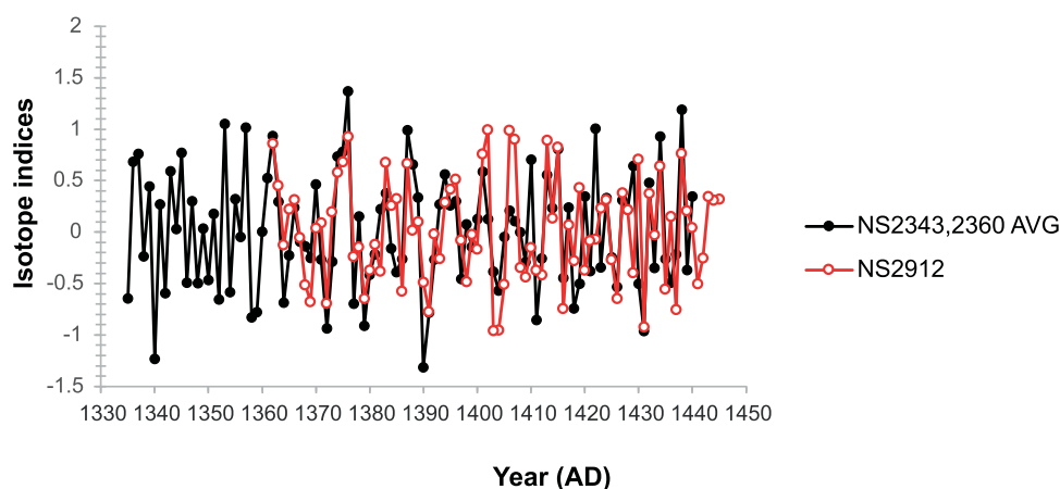
Figure 3. Visual comparison of the oxygen isotope series F114.2_NS2912 and the isotope mean of dated timbers P5.5_NS2343 and P16.1_NS2360, positioned at the date of best match AD 1335 to AD 1445 (Student's t = 6.51 1/p > 1 Million, IF > 1000 ). Twelve annual rings (not measured isotopically) at the end of NS2912 with possible bark edge imply a felling date of AD 1457B? (image: N.J. Loader)
