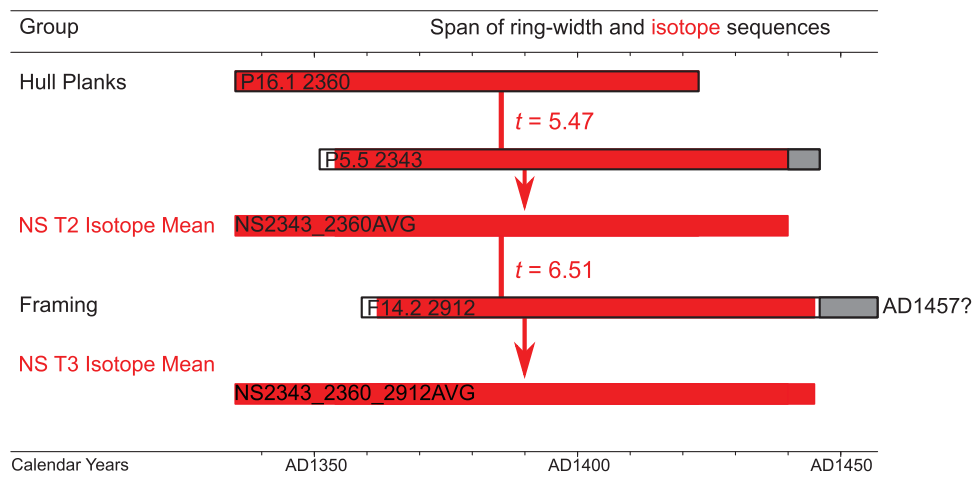
Figure 2. Bar diagram of original ring-width series (black outline with sapwood shaded grey) and isotope series (red) for the two hull plank samples, correlation between these two isotope series (Student's t = 5.47 ), construction of two-timber isotope mean, and correlation of isotope series from framing samples against it (Student's t = 6.51 ), and construction of three-timber isotope mean. Framing ring-width series absolutely dated with a possible bark edge date of AD 1457B? (image: N. Nayling).
