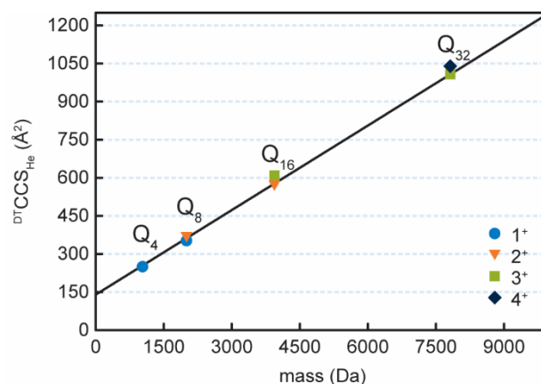
Fig. 4 Evolution of the collisional cross section ( {}^{\text{DT}}\text{CCS}_{\text{He}} ) as a function of the Q n mass. The linear regression ( R^2 = 0.99 ) indicates a perfectly cylindrical shape.
