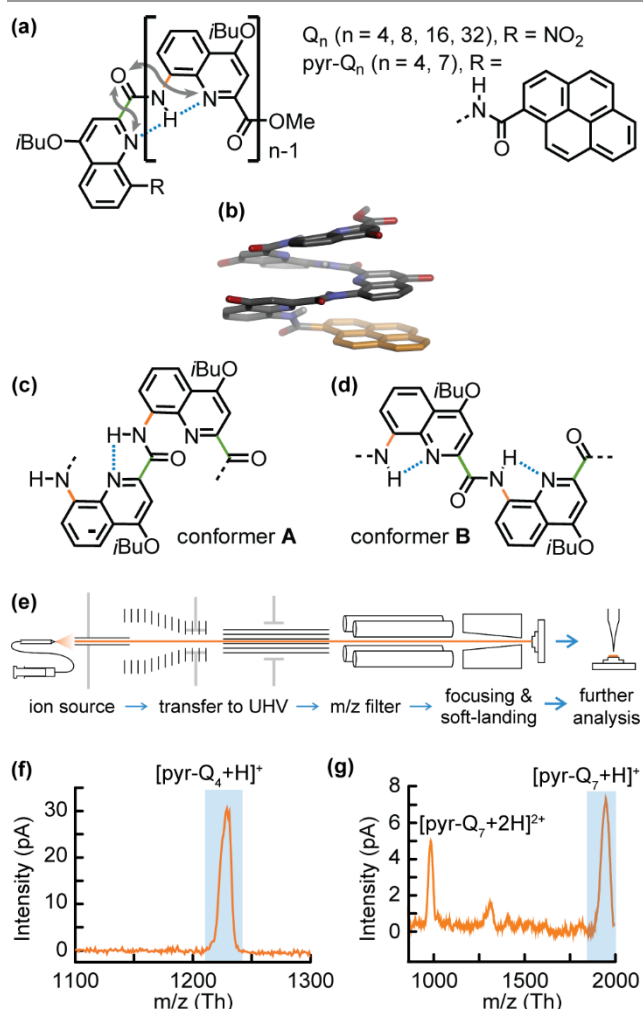
Fig. 1 (a) Chemical formula of Q n and pyr-Q n foldamers. Blue dotted lines point out hydrogen bonds and grey arrows show electrostatic repulsion. The aryl-amino and aryl-carbonyl bonds are coloured in green and orange, respectively. (b) Crystal structure of pyr-Q 4 (isobutyl groups and hydrogen atoms omitted for clarity). Ribbon structures of unfolded † molecule through either (c) rotation of the aryl-amino bonds (green) or (d) rotation of the aryl-carbonyl-bond (orange). (e) Schematic of the ES-CIBD system. Mass spectra prior to ES-CIBD of (f) pyr-Q 4 and (g) pyr-Q 7 . The m/z regions used for deposition emphasized with blue badges.
