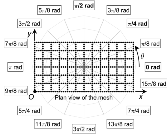
FIGURE 16 Orientations of the seismic waves used in the parametric analysis focusing on the directionality of earthquakes (plan view of the mesh).
