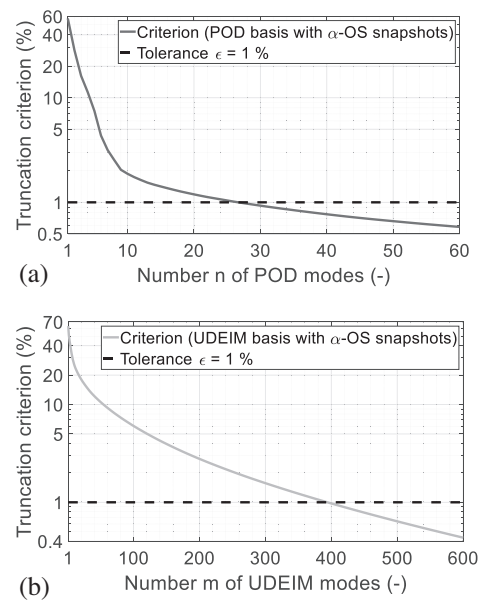
FIGURE 17 Criteria used to truncate the POD (a) and UDEIM (b) modal bases \Phi and \Psi .
