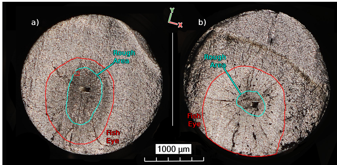
Figure 10a: Optical view of one side of two different fracture surfaces with internal crack propagation without contact with air i.e. under vacuum environment. a) specimen n°46). b) specimen n°59). The Rough-Area surrounds the initiation site and is comprised into a circular Fish-Eye zone. The red rectangle locates Figure 10b; based on Eq. 3, an average value of \Delta K \approx 6.7 \text{ MPa} \sqrt{\text{m}} is determined in this region.
