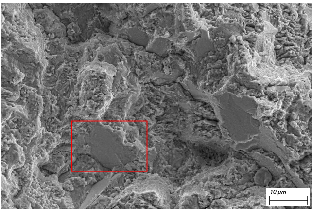
Figure 10b: SEM zoom on the rough area with facets separated by granular zones. The red rectangle locates Figure 10c.
