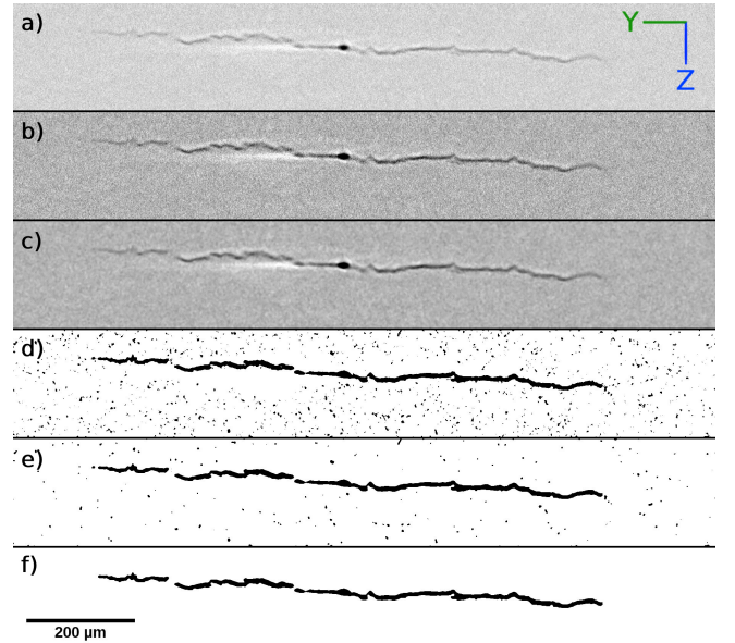
Figure 13: Successive steps of the thresholding protocol for a reconstructed slice of an internal crack after 4.4 \times 10^7 cycles of propagation under vacuum with a stress amplitude of 330 MPa (specimen n°46). The cutting plane of this section is represented in Figure 8. a) Initial grey level image. f) binary image after the thresholding protocol. See the text for a detailed explanation of the successive steps (b to e). All the pictures have the same scale as f).
