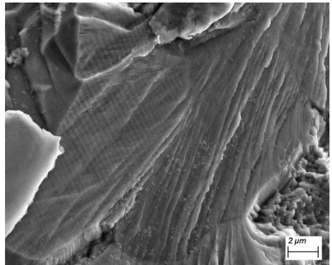
Figure 11f: SEM zoom on a facet from the bright zone showing extensive striations located in the yellow rectangle of Figure 11a.
