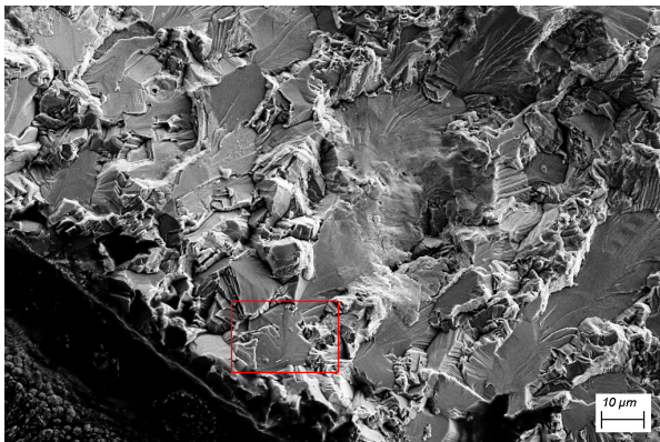
Figure 11b: SEM zoom on the black area with crystallographic aspect located in the red rectangle of Figure 11a. The red rectangle locates the Figure 11c.
