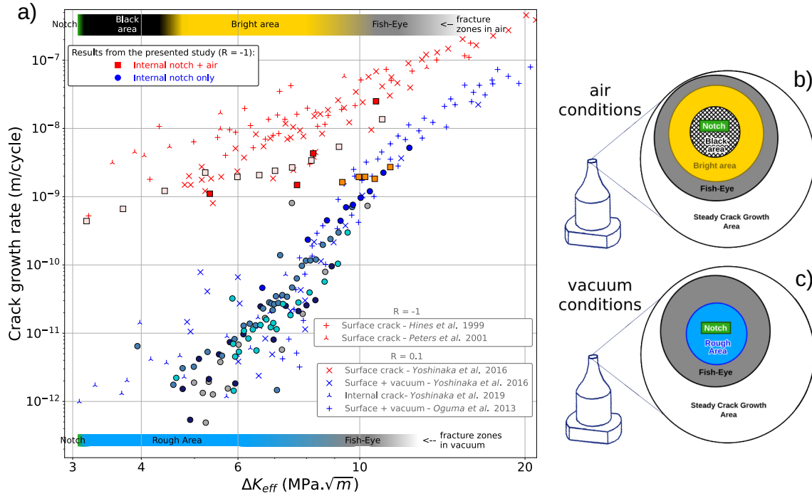
Figure 9: (a) Crack growth rate data of the tested specimens in a Paris diagram. Data from the cited studies were all run at "low" loading frequency (between 30 and 400 Hz). Table 2 links each marker type with a specimen. The SIF range corresponding to the different regions of the fracture surfaces in vacuum and in air are shown by the coloured bars respectively at the bottom and at the top of the curve as explained in Section 4.4. Scheme of the fracture surface for a crack which propagated in air (b) and vacuum (c) environment.
