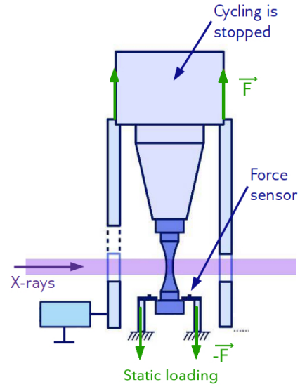
Figure 1b: \mu CT acquisition mode of the machine
