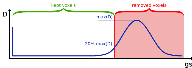
Figure 14: Typical grey level histogram used to determine the threshold value applied to a \mu CT stack.
