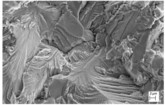
Figure 11d: SEM zoom on the bright zone with planar aspect located in the yellow rectangle of Figure 11a.
