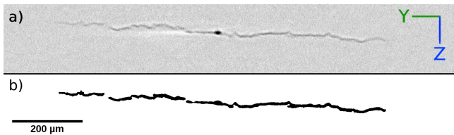
Figure 7: a) Initial grey level of a reconstructed slice of an internal crack after 4.4 \times 10^7 cycles of propagation under vacuum with a stress amplitude of 330 MPa (specimen n°46). b) Binary image after the thresholding protocol (cf. Appendix B) for the same slice. The location of this section in the 3D volume is represented in Figure 8.
