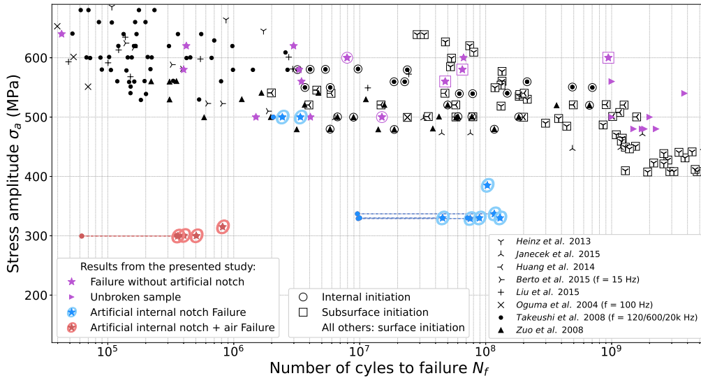
Figure 5a: Wöhler diagram comparing results from this work and from literature. The horizontal dashed lines represent the number of cycles between the crack first detection and final failure (values in Table 2).
