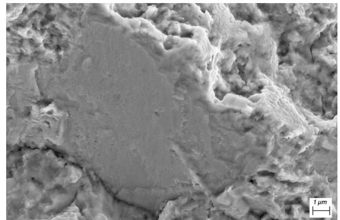
Figure 10c: SEM zoom on a facet located in the rough area.
