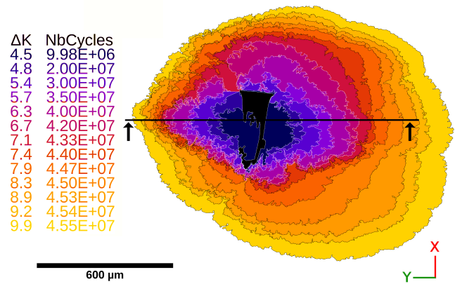
Figure 8: Crack shape projections at different propagation stages on a plane perpendicular to the loading direction. The stress amplitude is 330 MPa with a vacuum environment (specimen n°46). The cutting plane indicated by arrows corresponds to the section depicted in Figure 7. The displayed Stress Intensity Factor range \Delta K is calculated as detailed in Section, 4.3.
