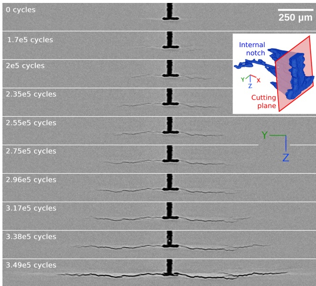
Figure 6: Reconstructed tomographic slices showing the propagation of an internal crack in contact with air - stress amplitude of 300 MPa and loading direction parallel to Z (specimen n°53). The chimney which brings the air from the top to the internal notch is visible on the slices.
