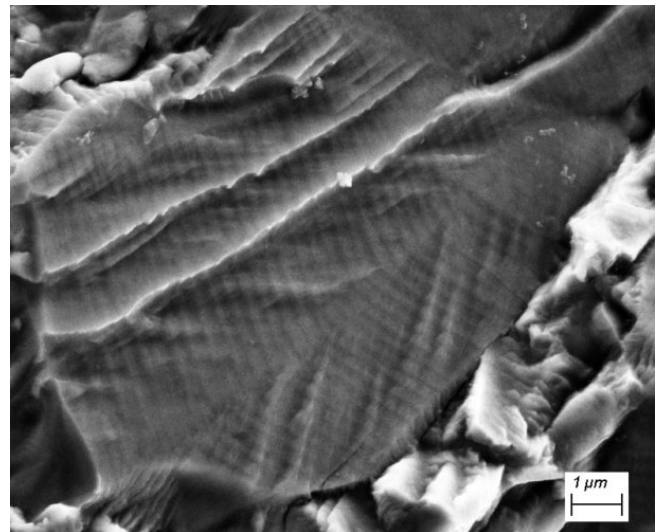
Figure 11e: SEM zoom on a facet from the bright zone showing extensive striations located in the yellow rectangle of Figure 11a.
