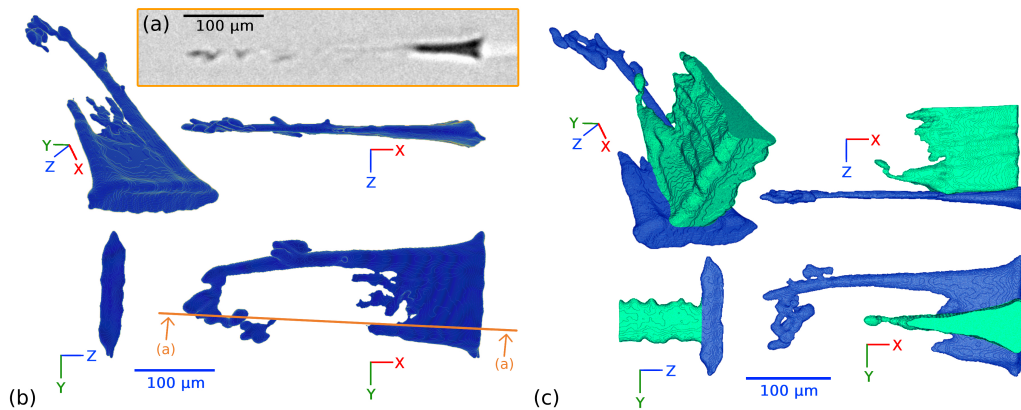
Figure 4: (a) Section of a notch without the chimney. 3D views of an internal notch (b) without and (c) with the chimney which can bring air to the internal crack. The chimney is displayed in green. (The loading direction is along z .)
