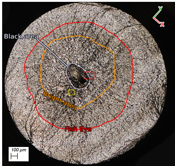
Figure 11a: Optical view of the fracture surface containing an internal crack which propagated under air environment (specimen n°48). A black area surrounds the initiation site and is comprised within a bright area which is itself in the Fish-Eye zone. The red rectangle locates Figure 11b. Figures 11d, 11e and 11f are located in the yellow rectangle where the value of the SIF range is estimated at \Delta K \approx 5.4 \text{ MPa} \sqrt{\text{m}} (Eq. 3).
