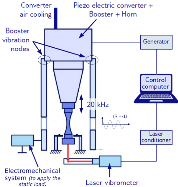
Figure 1a: Cycling mode of the machine
