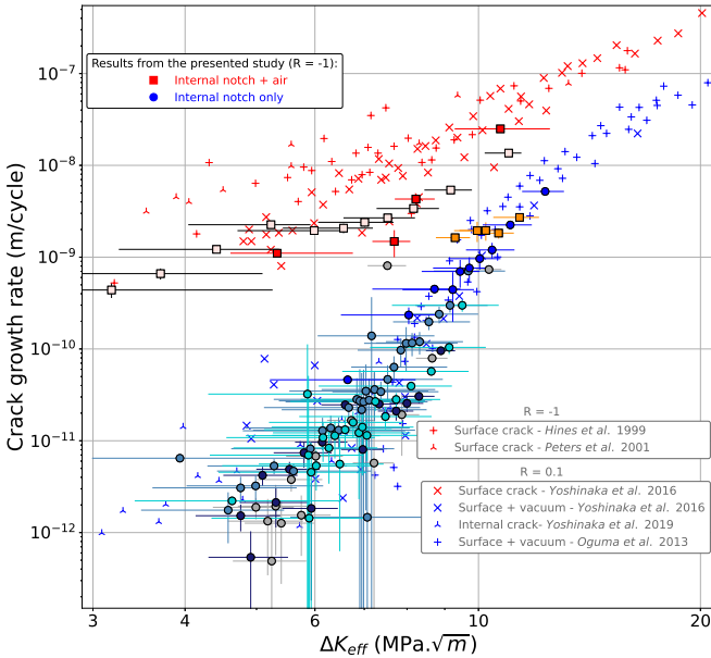
Figure 12: Experimental data of this study in a Paris diagram with the illustration of uncertainties (horizontal and vertical bars) compared with literature data (for which uncertainties are unknown).
