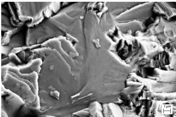
Figure 11c: SEM zoom on a facet from the dark zone located in the red rectangle of Figure 11b.
