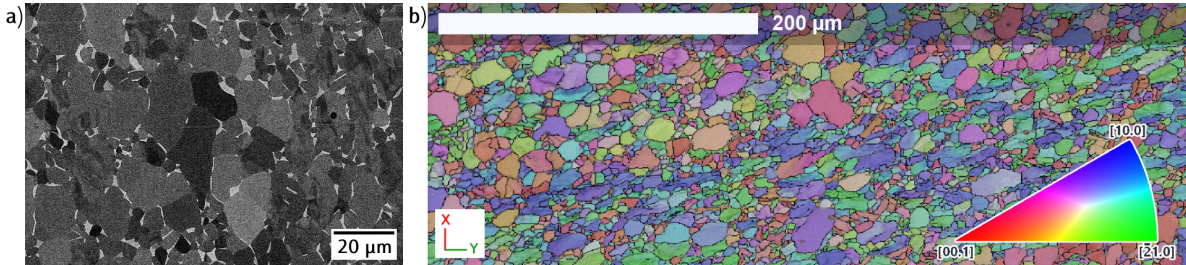
Figure 2: Ti64 microstructure observed with a) SEM back-scattered b) EBSD (map along the rolling direction Z).
