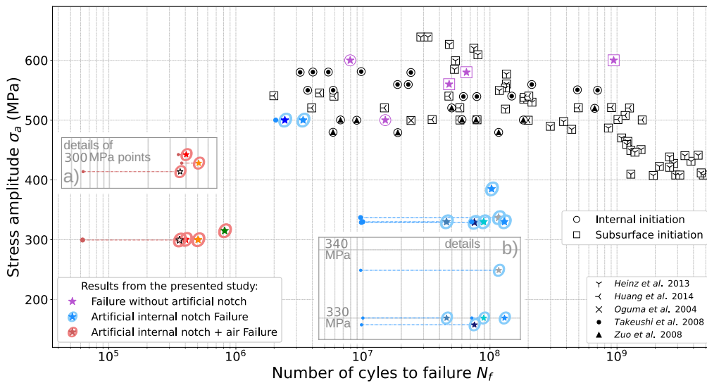
Figure 5b: Wöhler diagram comparing results from this work and from literature for internal or subsurface initiation only (no surface crack initiation). The specimens color code is given in Table 2. All points in inset a) have a 300MPa stress amplitude whereas inset b) presents points with different stress amplitudes.
