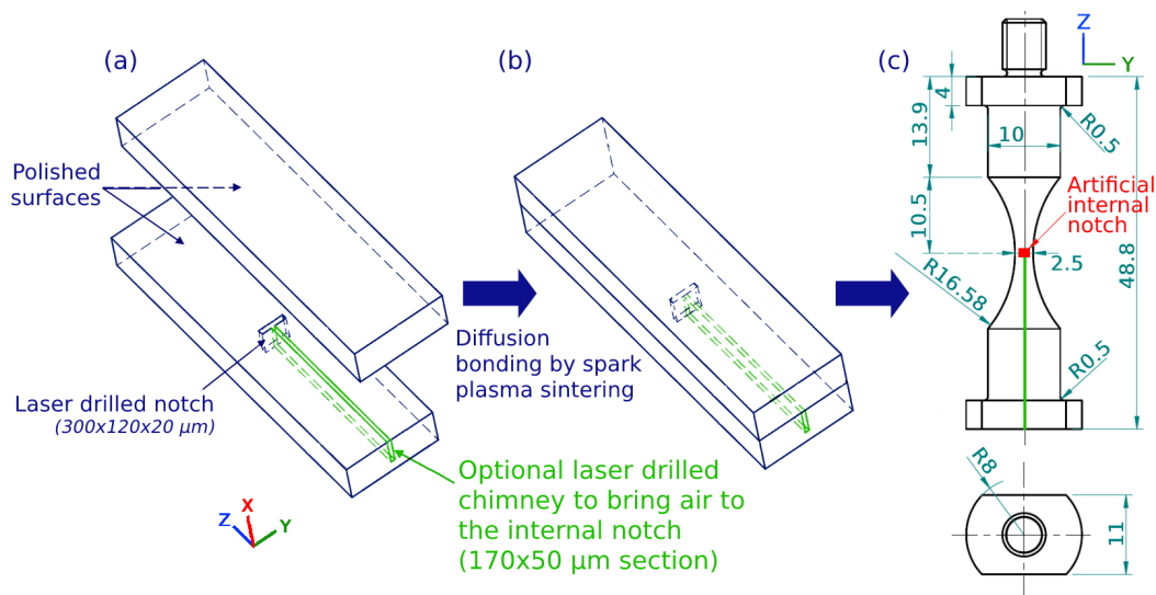
Figure 3: Specimen fabrication process: a) one half-sheet with an artificial notch is sintered with another unnotched half-sheet. b) sintered sheet used to manufacture the specimen. c) final specimen geometry (dimensions in mm). The green chimney is optional and can be added to bring air to the internal notch.
