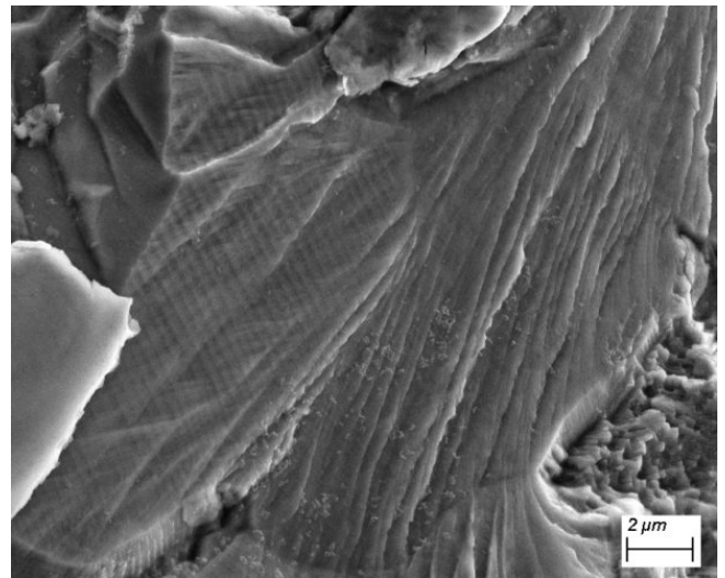
Figure 11f: SEM zoom on a facet from the bright zone showing extensive striations located in the yellow rectangle of Figure 11a.
