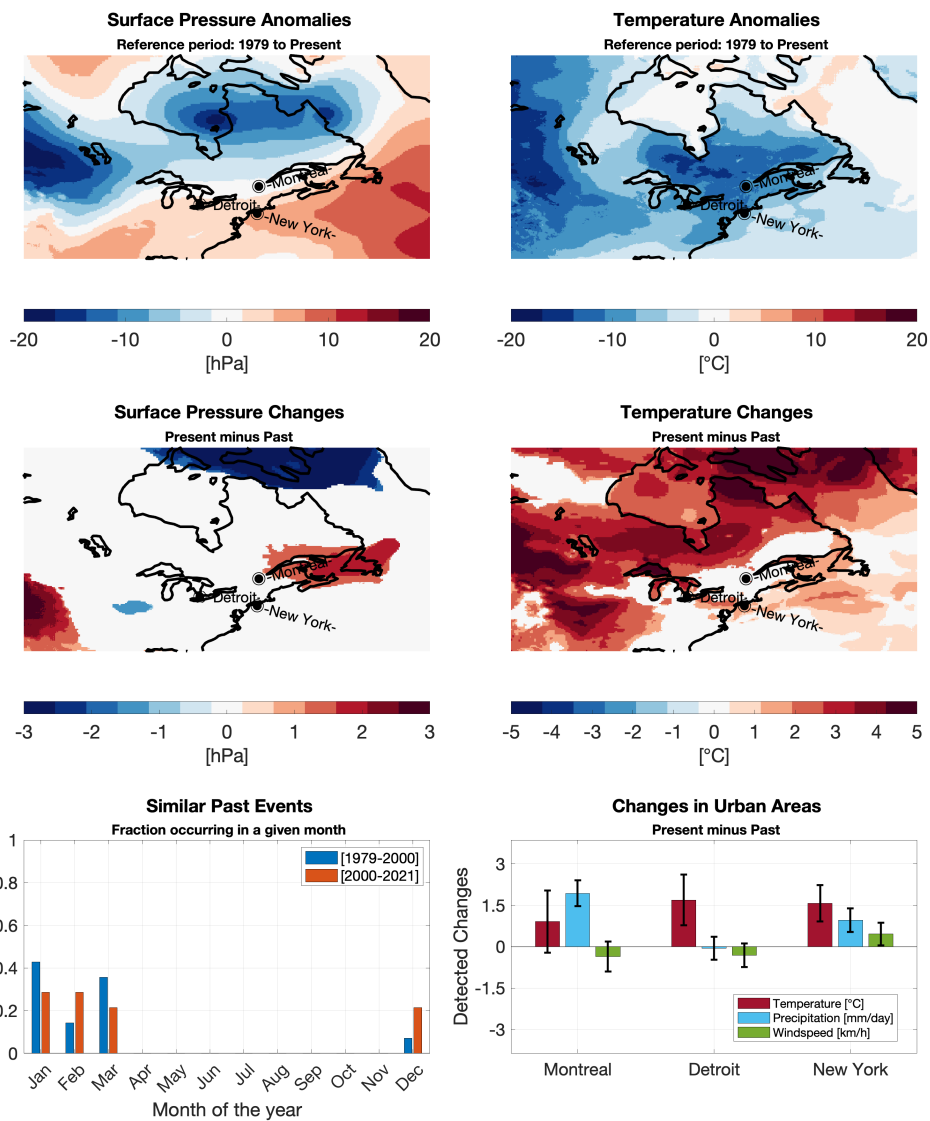
Figure 3. ClimaMeter output for 2022/12/21-26 North American Winter Storm.
