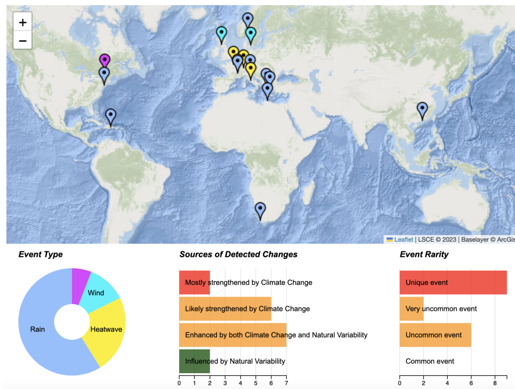
Figure 2. Screenshot of the Event Dashboard appearing in the ClimaMeter website, with extremes analyzed up to end of October 2023.
