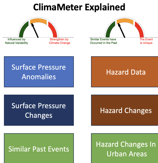
Figure 1. Schematic illustration of the ClimaMeter figure output.
