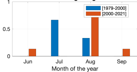
Figure 5. ClimaMeter output for 2023/08/20-23 Late Summer French Heatwave.
