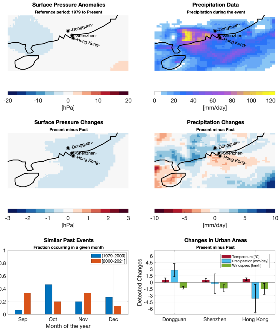
Figure 4. ClimaMeter output for 2023/09/08 Guangdong - Hong Kong Floods
