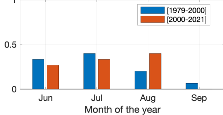
Figure 6. ClimaMeter output for 2023/07/05 Storm Poly in Northern Europe
