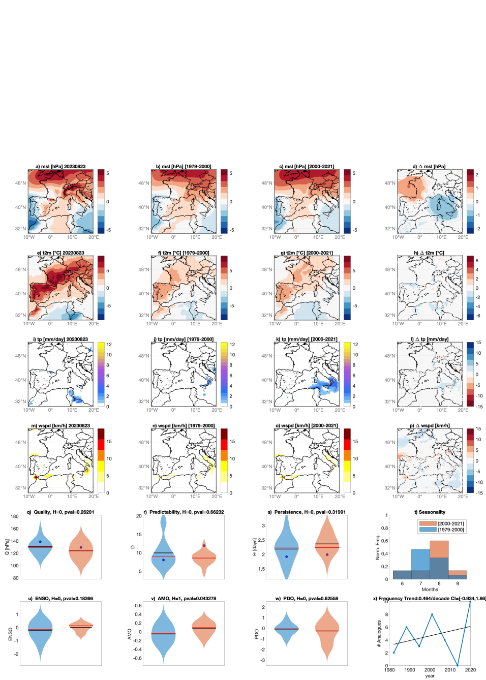
Figure A6. 2023/08/20-23 Late Summer French Heatwave. As in Figure A5 but for ERA5 data.
