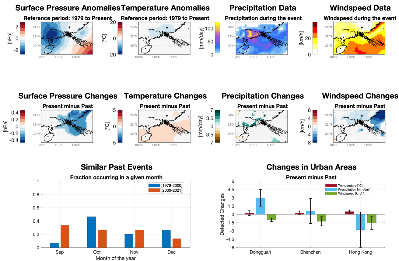
Figure 4. ClimaMeter output for 2023/09/08 Guangdong - Hong Kong Floods. See Figure 1 for an explanation of the different panels.
