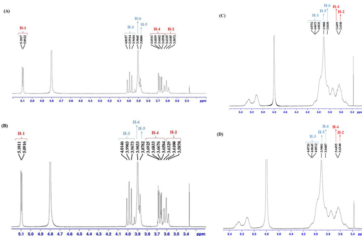
Figure 3 - ^1\text{H} NMR spectra obtained for \beta -CD (A), PHY/ \beta -CD (B), SB-E- \beta -CD (C) and PHY/SB-E- \beta -CD (D) in \text{D}_2\text{O} .
