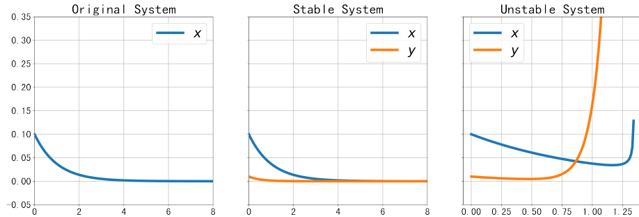
Fig. 1: Plot of the original equation, (3), and (4) with initial condition \mathcal{X}_0 = [x_0, y_0 = x_0^2] = [0.1, 0.01] . Numerical method: “LSODA” (uses hybrid Adams/BDF method with automatic stiffness detection) in scipy.integrate.solve_ivp package [22,29].
