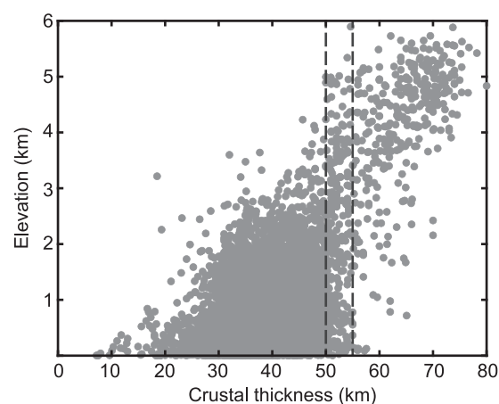
Fig. 10. Elevation vs. crustal thickness for all continental regions. Crustal thickness data is from the Crust 1.0 model ( https://igppweb.ucsd.edu/~gabi/rem.html ; Laske et al. , 2013) and elevation data is from the 1 arc-minute ETOPO1 global relief model for bedrock ( https://www.ngdc.noaa.gov/mgg/global/ ). Vertical dashed lines are drawn to bracket the elevation range of 50–55 km-thick crust.
