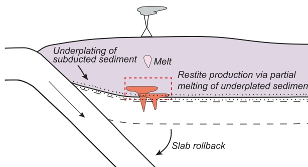
Fig. 4. Cartoon depicting scenarios leading to the production of (a) density-unstable and (b) density-stable residues.
