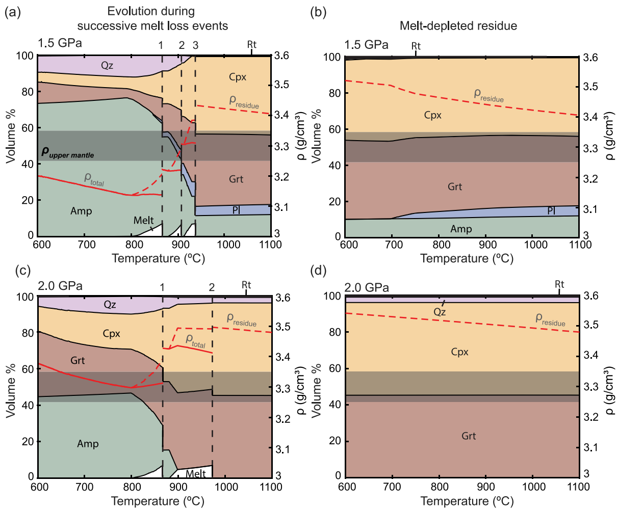
Fig. 6. Volume % vs temperature plots for an average water-undersaturated arc basalt undergoing partial melting at 1.5 GPa and 2.0 GPa. (a, c) Open-system partial melting and cyclic melt extraction at 7 vol.% (MCT). Dashed vertical lines represent melt loss events. (b, d) Phase equilibria of the melt-depleted residue. Densities of the total assemblage (solid red line) as well as the residual mineralogy (dashed red line) are shown with corresponding values on the right y-axis. The gray region represents the average density of the upper mantle (3.25–3.35 g/cm 3 ). See Fig. 3 for mineral abbreviations.
