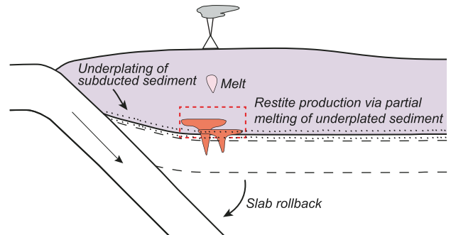
Fig. 4. Cartoon depicting scenarios leading to the production of (a) density-unstable and (b) density-stable residues.
