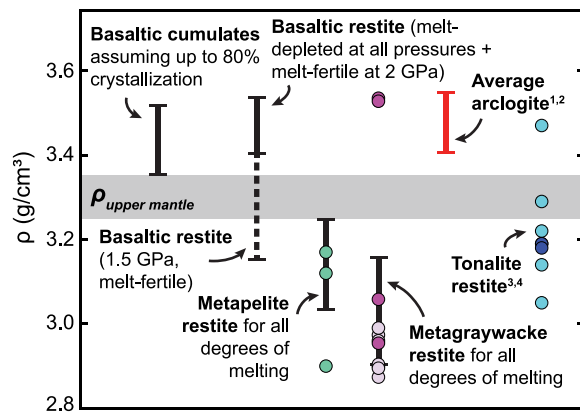
Fig. 5. Summary diagram showing the density ranges (in black) of basalt-derived cumulates as well as basaltic, metapelitic, and metagraywacke restites generated by our thermodynamic models. Densities of basaltic restites are broken up into those that are density-unstable (melt-depleted restites at all pressures + melt-fertile restites at 2 GPa; solid line) and those that extend to densities lower than that of the mantle (only melt-fertile restites at 1.5 GPa; dashed line). For comparison, shown in red is the average density range of natural arclogites from Ducea (2002) 1 and Jagoutz & Schmidt (2013) . 2 Light blue points are tonalite restites formed experimentally by Patiño Douce (2005) 3 at 1.5 and 2.1 GPa from 940–1060°C. The one light blue point with a density greater than the upper mantle was partially melted at 1060°C, the highest investigated temperature. Dark blue points are natural tonalite restites from Hacker et al. (2005) . 4 Shown in green are the densities of sanidine eclogites from the Pamir interpreted by Hacker et al. (2005) as metapelitic restites. Purple points are restites of biotite-bearing, Ti-rich, Al-poor metagraywacke experimentally melted at 1.5 and 2 GPa with densities calculated using Abers & Hacker (2016) . Dark purple points are densities of biotite gneiss-derived restites from Patiño Douce & Beard (1995) . Density-unstable restites form where high temperatures (>975°C) cause full consumption of biotite. Light purple points are from Auzanneau et al. (2006) .
