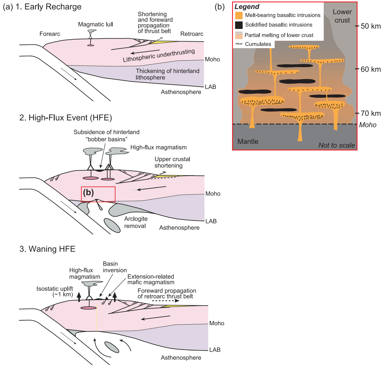
Fig. 1. (a) Cartoon depicting the stages of the Cordilleran cycle. During (1) early recharge, retroarc shortening delivers melt-fertile lithosphere to the subarc region. Melting of this fertile lithosphere in the deep crustal hot zone (red box) leads to (2) high-flux magmatism, which generates a dense residual arclogitic root in the subarc lower crust. This root takes up space in the mantle wedge, restricts further retroarc underthrusting, and causes surficial subsidence and 'bobber basin' formation. Because it is gravitationally unstable, the root founders into the asthenosphere. During the (3) waning stage of the high-flux event, lithospheric foundering and concomitant asthenospheric upwelling cause rapid surficial uplift, hinterland extension, and local basaltic volcanism. Creation of space in the mantle wedge allows renewed horizontal shortening, and the cycle begins again. Modified from DeCelles et al. (2015a). (b) Schematic of a deep crustal hot zone (Annen et al. , 2006), the locus of intrusion of hot, hydrous mantle-derived basalt into the lower crust of an active arc. Here, fractional crystallization and partial melting act in concert to form the intermediate magmas of Cordilleran upper crustal batholiths. Based on Cashman et al. (2017).
