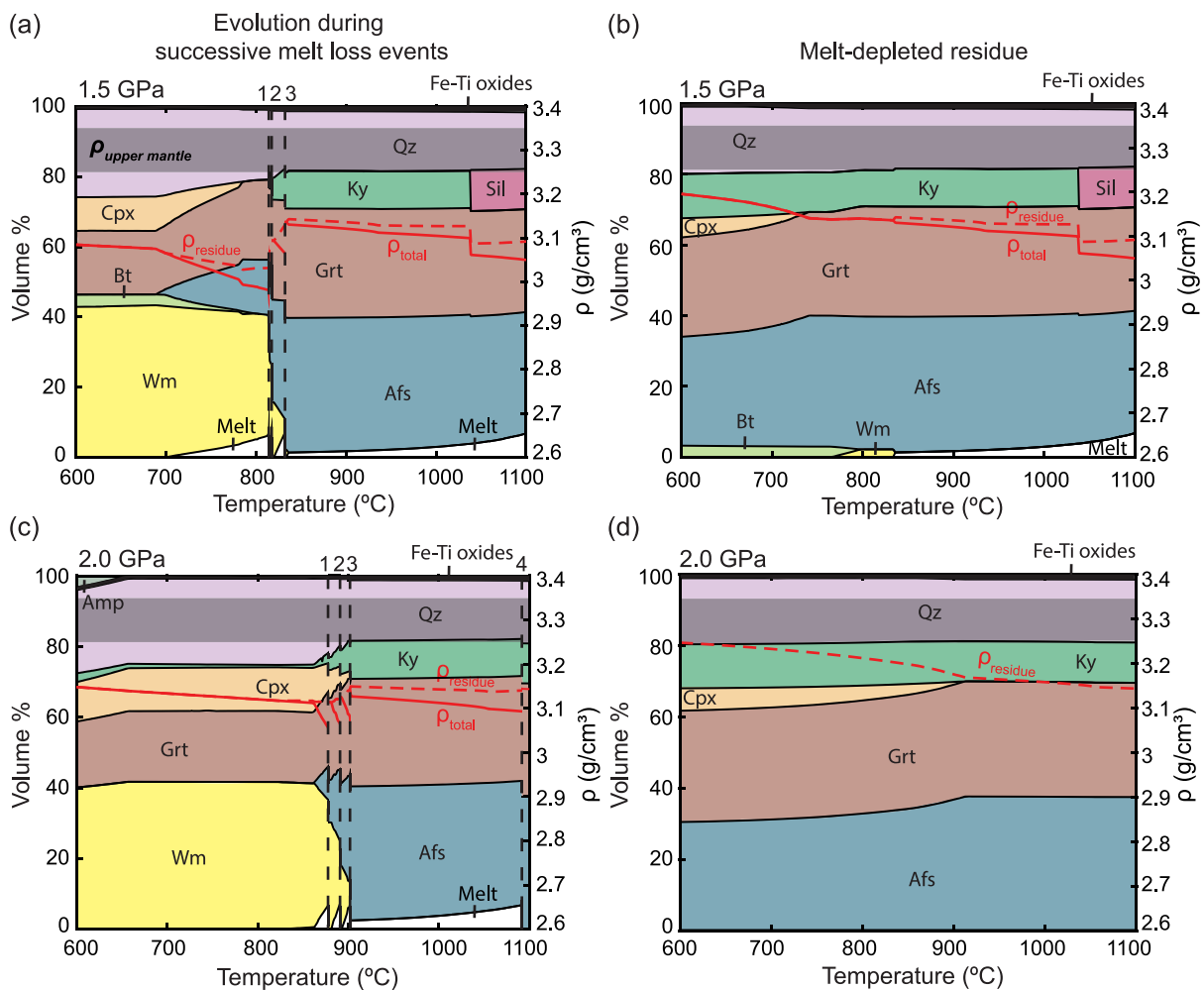
Fig. 7. As in Fig. 6, but for an average water-undersaturated metapelite. See Fig. 3 for mineral abbreviations.
