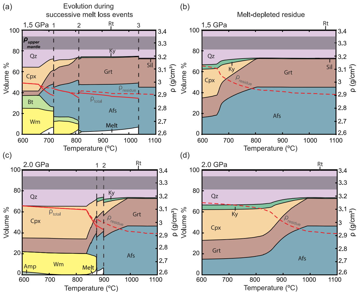
Fig. 8. As in Figure 6, but for an average water-undersaturated metagraywacke. See Fig. 3 for mineral abbreviations.
