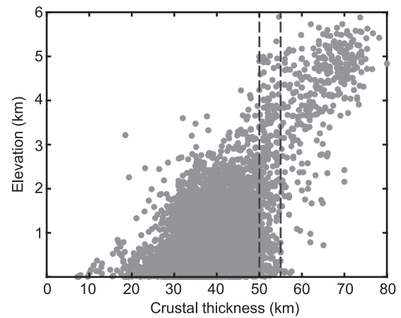
Fig. 10. Elevation vs crustal thickness for all continental regions. Crustal thickness data is from the Crust 1.0 model ( https://igppweb.ucsd.edu/~gabi/rem.html ; Laske et al. , 2013) and elevation data is from the 1 arc-minute ETOPO1 global relief model for bedrock ( https://www.ngdc.noaa.gov/mgg/global/ ). Vertical dashed lines are drawn to bracket the elevation range of 50–55 km-thick crust.
