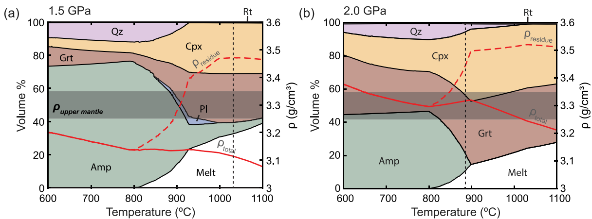
Fig. 3. Volume % vs temperature plots for an average water-undersaturated arc basalt at (a) 1.5 GPa and (b) 2.0 GPa. Densities of the total assemblage (solid red line) as well as the solid residual assemblage (dashed red line) are shown with corresponding values on the right y-axis. The gray region represents the average density of the upper mantle (3.25–3.35 g/cm 3 ). The region to the right of the vertical dashed line is the temperature range at which the solid residue has an average arclogitic mineralogy (equal proportions of garnet and clinopyroxene plus 0–10 vol.% amphibole; Ducea et al. , 2021a). Mineral abbreviations for all figures are: Wm = white mica, Afs = alkali feldspar, Bt = biotite, Ky = kyanite, Sil = sillimanite, Amp = amphibole, Pl = plagioclase, Grt = garnet, Cpx = clinopyroxene, Qz = quartz, Rt = rutile.
