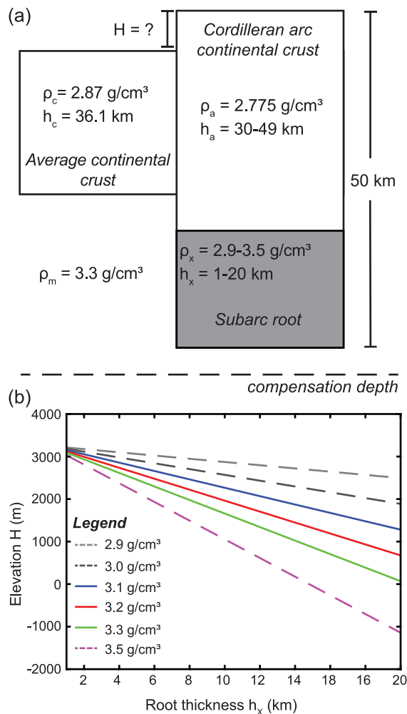
Fig. 9. (a) Cartoon showing the density and thickness structure of a Cordilleran arc (right) relative to average continental crust (left). Shown in gray is the subarc lower crustal root, which may be composed of arclogite. We vary the thickness and density of the lower crust from 1–20 km and 2.9–3.5 g/cm 3 , respectively, while maintaining the crustal thickness of the bulk arc at 50 km. The upper crust of the arc is varied from 30–49 km and has a density of 2.775 g/cm 3 (Hacker et al. , 2015). The density and thickness of the average continental crust are taken, respectively, as 2.87 g/cm 3 (Lee et al. , 2015) and 36.1 km (Hacker et al. , 2015). The density of the upper mantle down to the compensation depth is assumed to be 3.3 g/cm 3 . (b) Plot depicting how the elevation of the arc ( H ) relative to average continental crust varies as a function of the thickness (1–20 km) and density (2.9–3.5 g/cm 3 ) of the lower crustal root. See text for detailed explanation.
