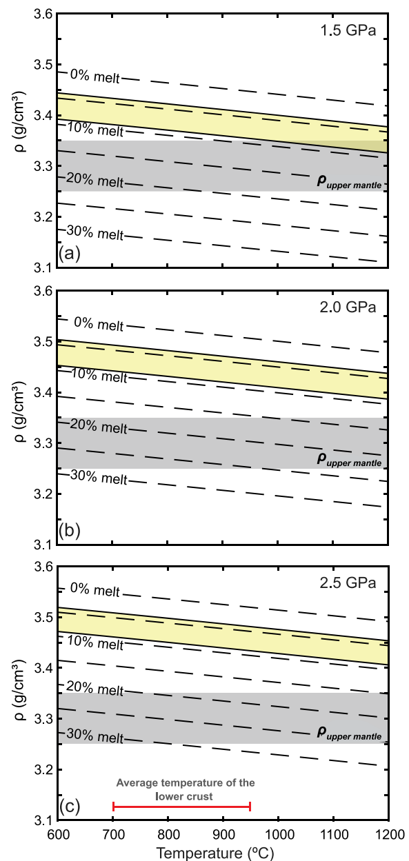
Fig. 2. Density of the refractory subarc root vs temperature for different percentages of trapped intermediate melt at (a) 1.5, (b) 2.0, and (c) 2.5 GPa. Shown in gray is the average density of the upper mantle (3.25–3.35 g/cm 3 ). The yellow region highlights the amount of melt seismically detected in the lower crust of the central Andean Cordillera (Delph et al. , 2017). The average temperature of the lower crust (700–950°C) is outlined in red.
