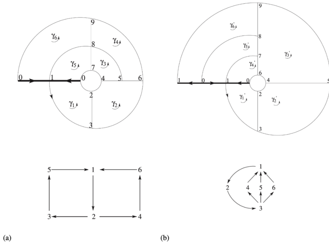
Figure 17. Templexes for (a) the spiral and for (b) the funnel attractors corresponding to the structures in phase space shown in Fig. 15a and b, respectively. Cell complexes (above) are shown as planar diagrams, with the convention that points (0-cells) and segments (1-cells) with identical labels must be glued to each other. The digraphs provide the allowed connections between the polygons (2-cells) labeled \gamma_i for the spiral case and \gamma'_i for the funnel case, with i \in \mathbb{N} . The two cell complexes are homologically equivalent. Reproduced from Charó et al. (2022) with the permission of AIP Publishing.
