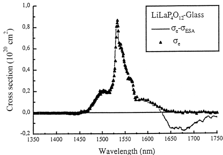
Fig. 5. \text{Er}^{3+} \sigma_e stimulated emission and \sigma_{esa} excited-state absorption cross-sections in the eye-safe range around 1535 nm.
