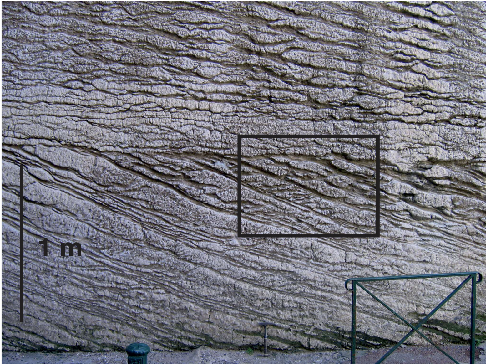
Fig. 18 – Typical facies of the unit 3 of the Bonifacio Member (B3 in Fig. 7) in the citadel of Bonifacio (Stop T2.2.2). The upper part of the picture corresponds to the toesets and bottomsets of the dunes. The nodular aspect in the flat bedded facies might be partly due to bioturbation by echinoids. In the lower part (black frame), the large dune foresets show a rhythmic pattern of accretion, with alternating thin- and thick beds, the latter showing internal upclimbing cross-lamination, that is created by superimposed dunes. These dunes are likely too high in the foreset to correspond to backflow bedforms. In the tidal interpretation, this might rather be the record of the subordinate tidal current. Modified from André et al. (2011).
