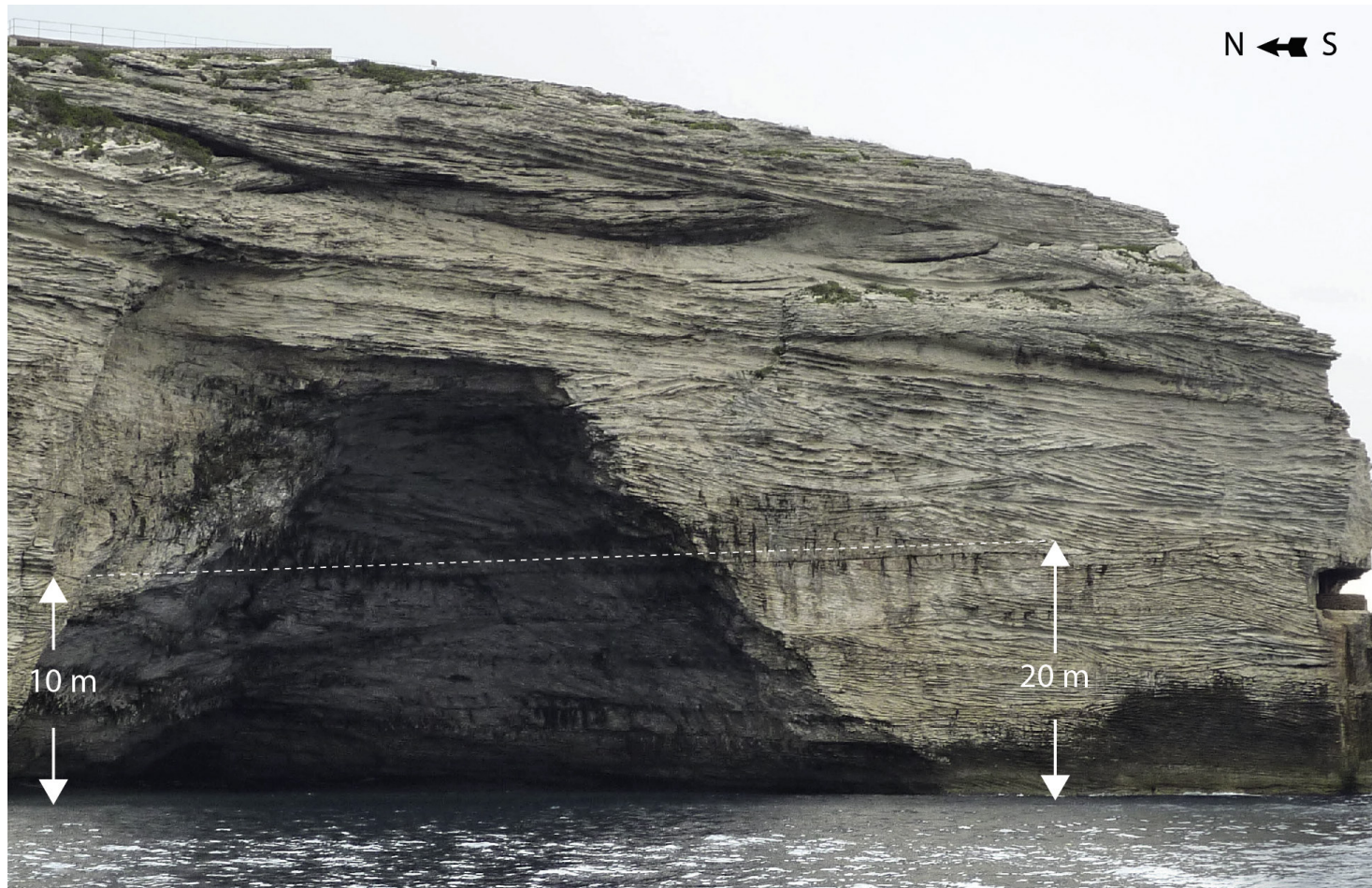
Fig. 20 - Large-scale architecture of the unit 3 of the Bonifacio Member at the entrance of the ria of Bonifacio (Stop T2.2.3). This spectacular outcrop, with a karstic cave in the middle, shows well the overall aggradation of the large dunes, with a flat, horizontal master-bedding, well expressed at the top of the cliff. The picture shows a discrete planar surface (dotted white line, placed above the real surface, to keep the latter visible), slightly oblique to the master-bedding, that separates packages of dune cross-sets. This surface suggests the presence of bedforms (bars?) of larger amplitude than the large dunes (larger than 10 m, which is the difference in elevation noted along the surface on this outcrop).
