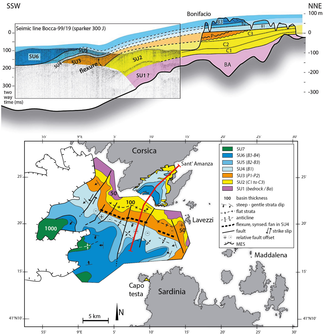
Fig. 5 – Top: Correlation of seismic units (SU) identified in Bonifacio Strait with Miocene stratigraphic units outcropping in the onshore part of the strait (Ba: Balistra, C: Cala di Labra, B: Bonifacio formations and members). Bottom: Geologic map of Miocene units based on reflection seismics (Quaternary cover, less than 20 m thick, not displayed). The location of the cross-section displayed above is indicated by the red line. MES: Messinian Erosion Surface. Modified from Reynaud et al. (2012a).
