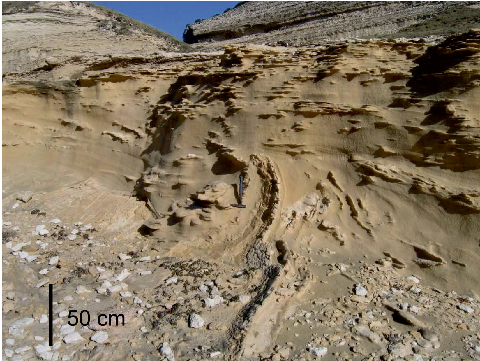
Fig. 13 - Syn-sedimentary soft-deformation in the middle part of Pertusato Member at stop T2.1.3 (modified from André et al., 2011). In the simplified description of the Pertusato Member by Reynaud et al. (2012a), this facies is included to the lower unit P1 (Fig. 7).
