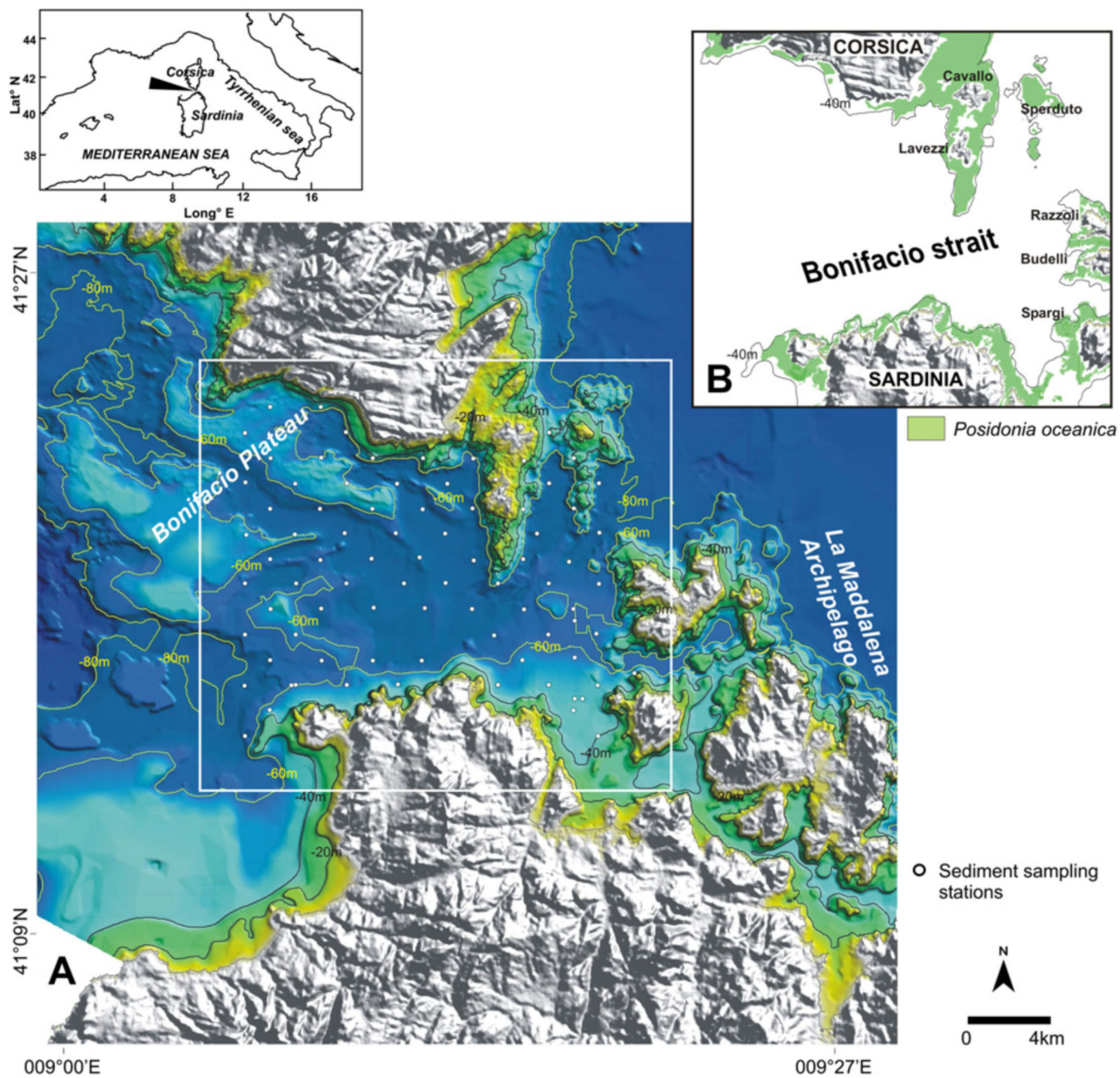
Fig. 4 – Morphology of the Corsican-Sardinian strait (modified from De Falco et al., 2011). A: The Bonifacio Plateau corresponds to the submarine top of the Miocene deposits that crop out onshore. It is dissected by karstic paleovalleys shaped during the Quaternary sea-level lowstands. The white box corresponds to the Posidonia meadows map in B. These green algae produce amounts of felt balls that accumulate in sheltered embayments. Razzoli, Budelli and Spargi islands belong to the Maddalena Islands. Lavezzi, Cavallo and Sperduto islands form the Lavezzi Islands.
