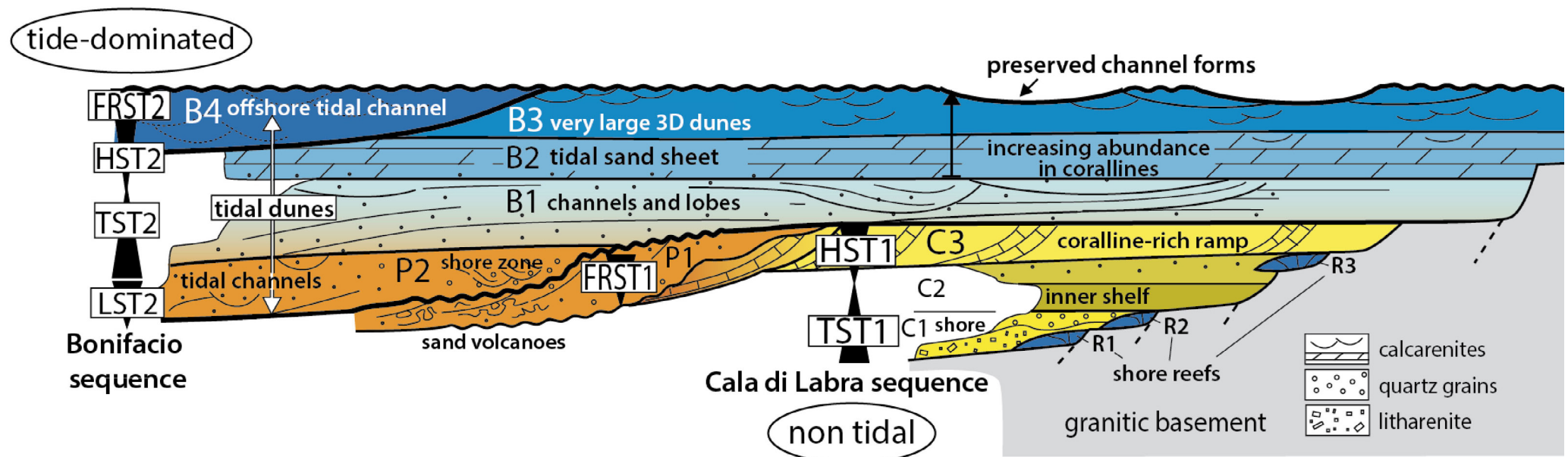
Fig. 7 – Sequence stratigraphic interpretation of the Miocene marine formations of Bonifacio (modified from Reynaud et al., 2012a). The Cala di Labra Formation comprises units C1 to C3. The Bonifacio Formation comprises the Pertusato Member (P1 and P2) and the Bonifacio Member (B1 to B4). This section is a synthetic sketch of the observations made on the southeastern basin border, from Cala di Labra to Anciennes Batteries.
