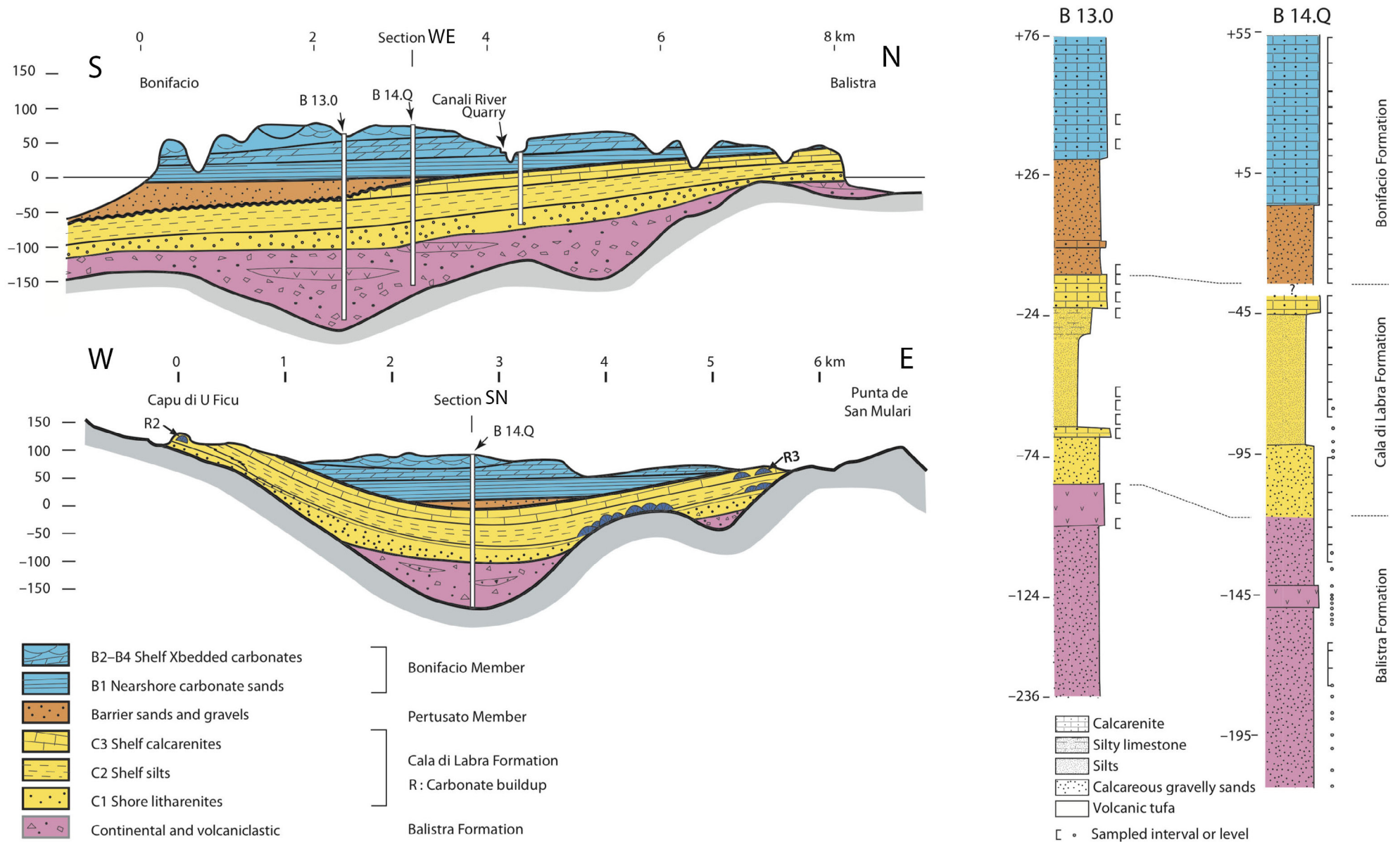
Fig. 6 – Cross sections of the onshore part of Bonifacio Basin (modified from Reynaud et al., 2012a). The section SN is the one displayed in Fig. 5 Top. The geometry of the stratigraphic units in subsurface is controlled by resistivity profiles and wells (B13 and B14). The logs were reconstructed based on cuttings from the wells. Note that the fold mostly predates deposition of the Bonifacio Member.
