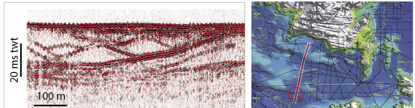
Fig. 8 – High-resolution sparker seismic profile showing cut-and-fill structures similar to the very-large 3D dunes in unit B3. Modified from Voisin (2013). The map on the right shows the location of the full profile. The red circle indicates the location of the displayed part.
