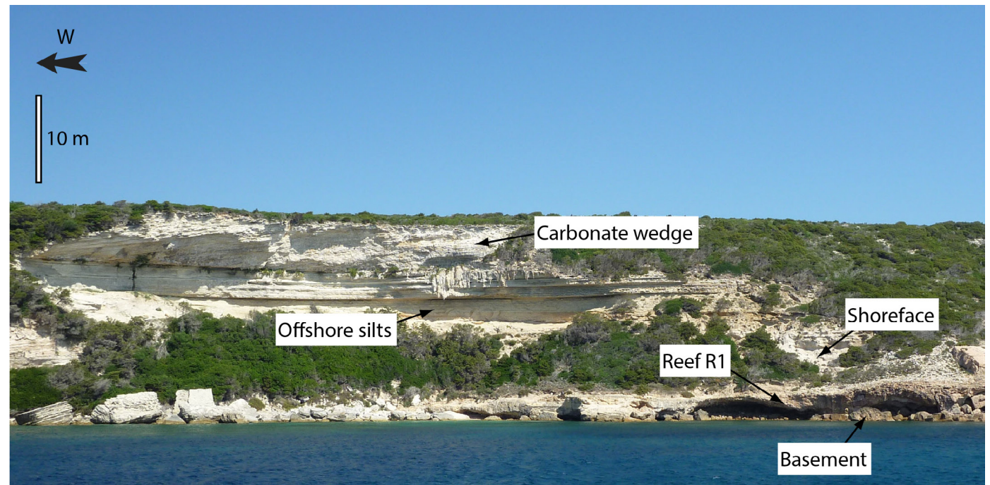
Fig. 12 – View of Cala di Labra Formation from the sea at Cala di Labra (Stop T2.1.2). The upper part will be seen to the left of the outcrop. This section is represented in Fig. 7 (offshore silts correspond to inner shelf facies, and carbonate wedge to coralline-rich ramp).
