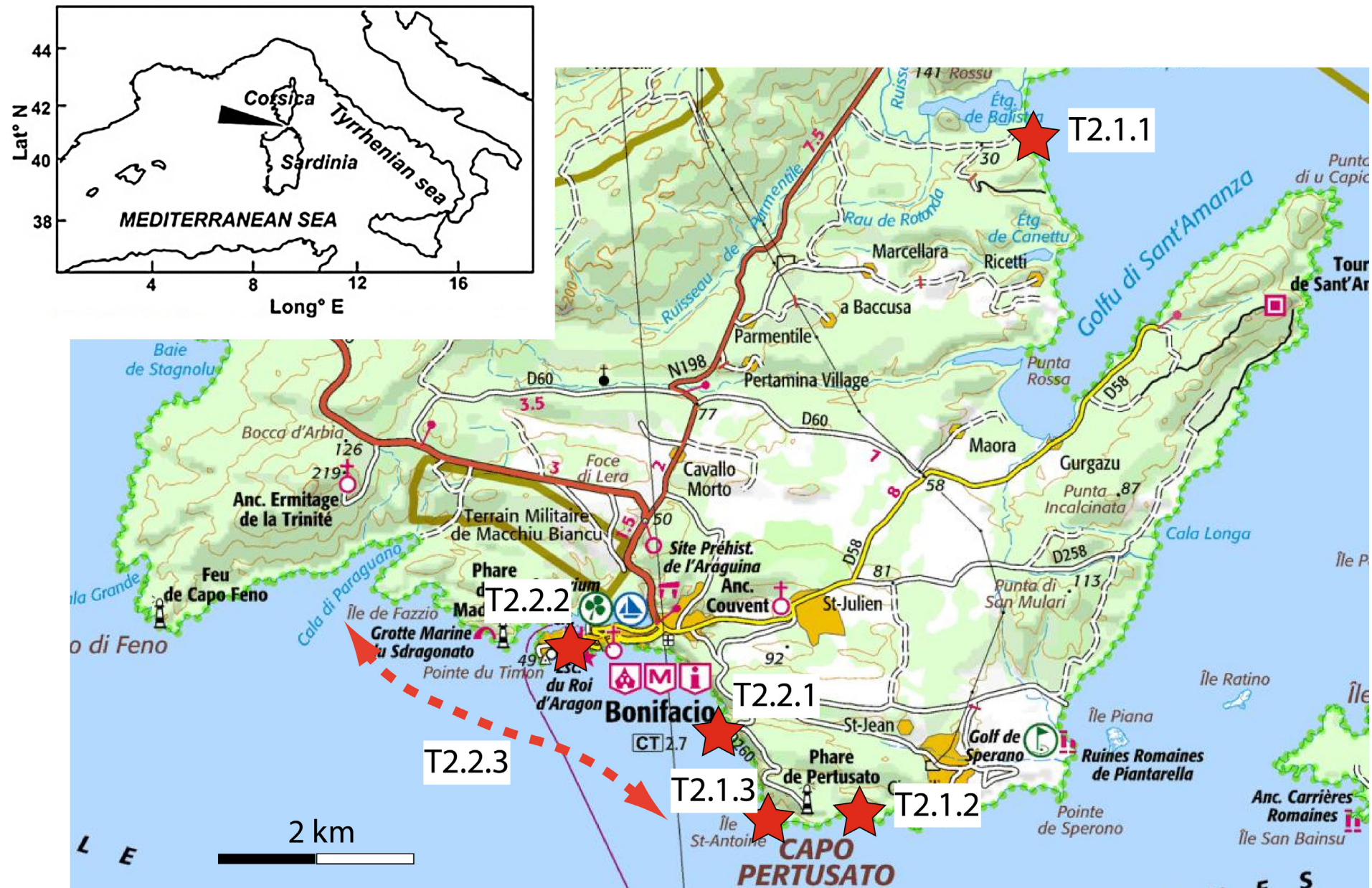
Fig. 1 – Part of the 1:100,000 IGN topographic map of southern Corsica, with the itinerary stops indicated. Dotted arrow in stop T2.2.3 indicates the coastal area covered by the boat trip. Source: IGN Top100 Ajaccio-Bonifacio. Inset map: location of Southern Corsica (arrow) in the Western Mediterranean.
