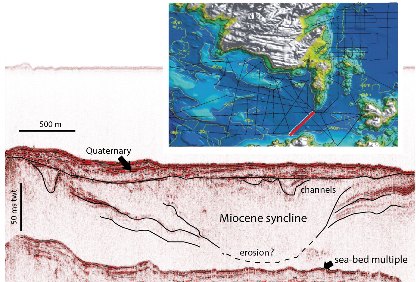
Fig. 9 – High resolution sparker seismic profile of the narrowest part of the strait, in about 75 m water depth. It shows a syncline of Miocene strata with channels incised at the top, beneath a thin cover of Quaternary deposits (modified from Museur, 2014). The syncline appears to be over-deepened by an intra-Miocene erosional unconformity. Reynaud et al. (2012a) interpret this feature as a tidal scour related to the Langhian sea-level fall.
